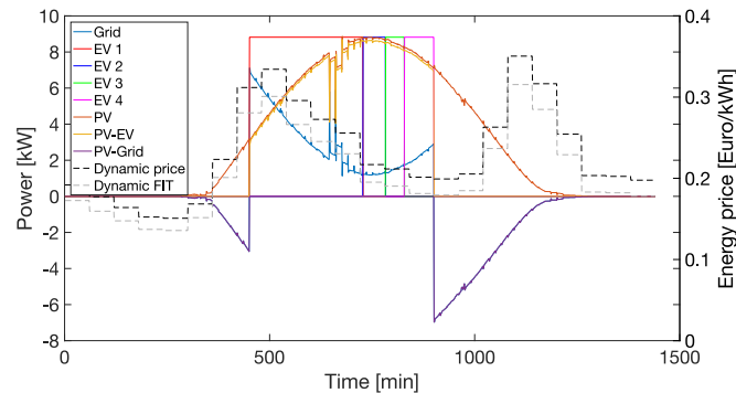
Fig. 4. Power allocation with dynamic FIT, 4 BEVs, uncontrolled charging.
