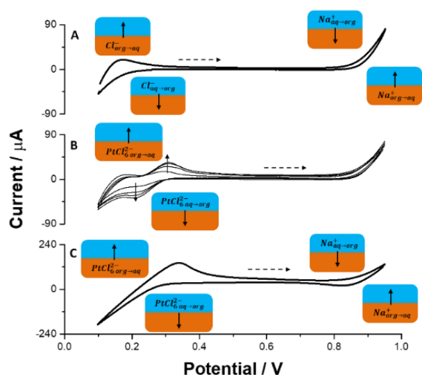
Figure 2. Ion transfer voltammograms recorded at the Liquid-liquid Interface formed between A – 10 mM NaCl (aq) // 10 mM BTTPATPBCl (org); B – 10 mM NaCl (aq) // x μM (x = 58; 116; 174 and 232 μM) BTTPA 2 PtCl 6 in 10 mM BTTPATPBCl (org) and C – 10 mM NaCl (aq) // 5 mM BTTPA 2 PtCl 6 (org). Scan rate was 10 mVs -1 ; dashed arrow indicate the direction of the forward scan.
