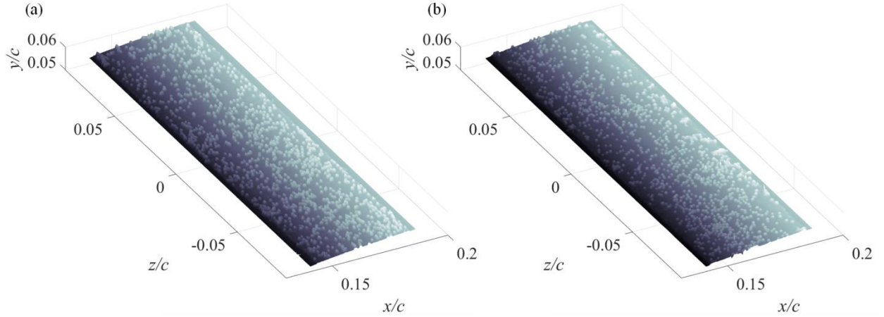
Fig. 2. Reconstructed surface roughness distribution by 3D scanning on the (a) suction and (b) pressure side.
