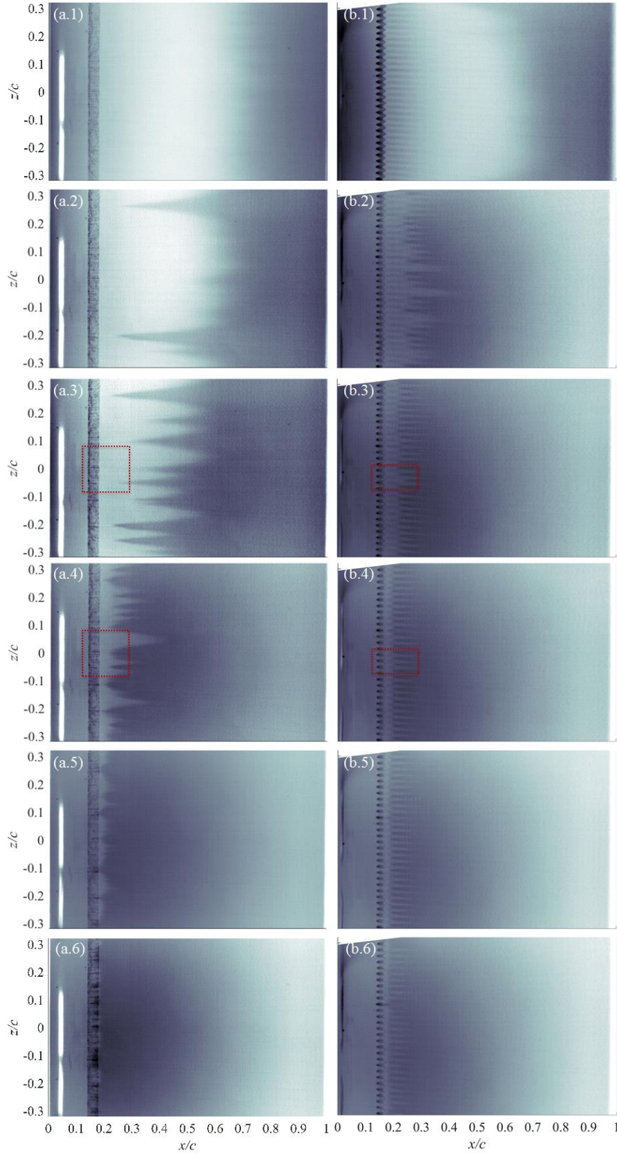
Fig. 4. Surface temperature distribution. (a) and (b) correspond to the grit and zigzag, respectively. (1)-(6) represent u_\infty = 16, 18, 20, 25, 30, \text{ and } 35 \text{ m/s} , respectively. The red box indicates hotwire measurement range.
