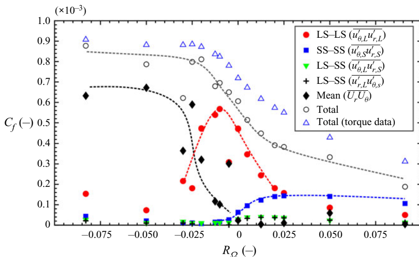
FIGURE 5. Contributions to the friction factor C_f associated with the mean flow and the instantaneous large-scale (LS) and smaller-scale (SS) velocity fluctuations in the TC gap at Re_S = 29\,000 . Their combined total (circles) is compared against the estimated based on the torque measurements of Ravelet et al. (2010) (triangles). The dashed lines are indicative of the trend in the data.
