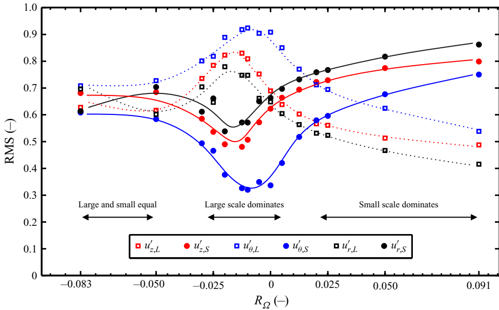
FIGURE 2. The r.m.s. of fluctuating large- and small-scale velocities versus R_\Omega at Re_S = 29\,000 . u'_z , u'_\theta and u'_r represent the fluctuating velocities in the axial, azimuthal and the radial directions, respectively. The second indices L and S (e.g. u'_{z,L} and u'_{z,S} ) represent the large- and smaller-scale components of the fluctuating velocity, respectively. The lines are included to guide the eye. The r.m.s. of fluctuating large- and small-scale velocities are normalized using the r.m.s. of the non-filtered fluctuations of each velocity component, e.g. u'_z . Horizontal arrows indicate the dominant scale in the different ranges of the rotation number.
