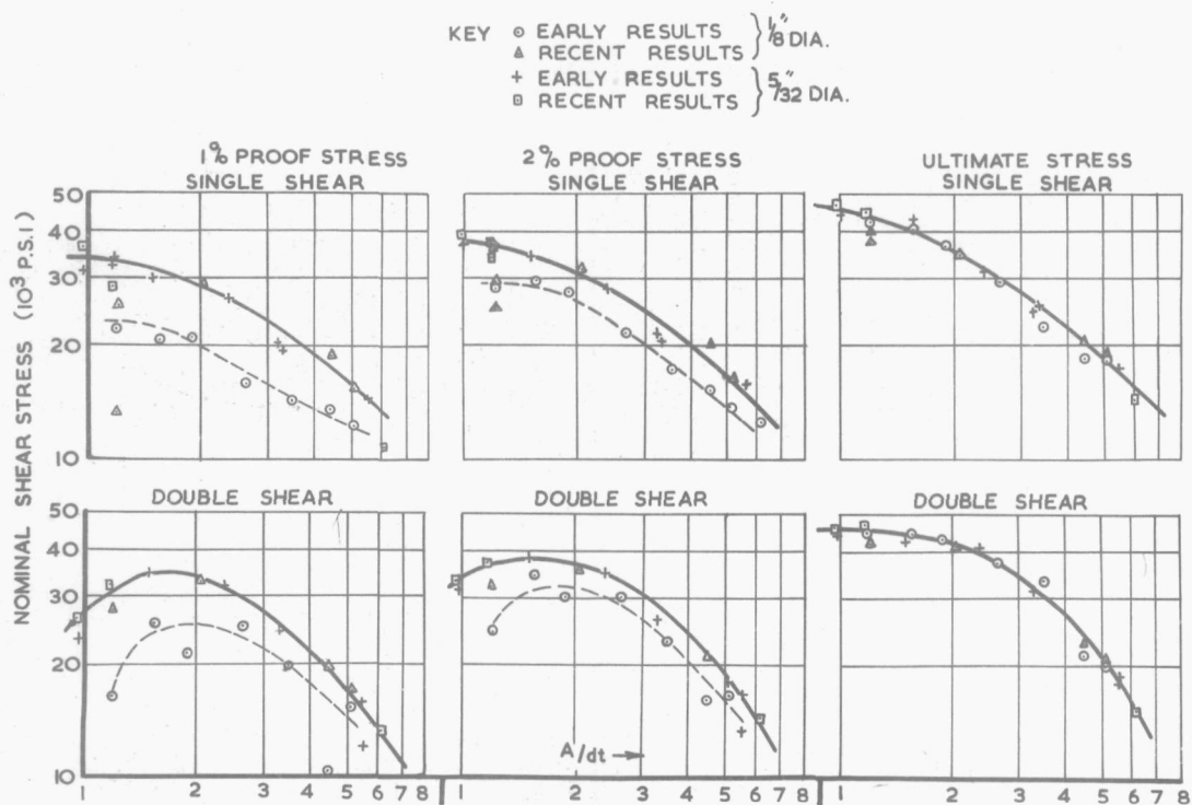
FIG. 4 NOMINAL SHEAR STRESSES & AREA RATIO PARAMETER
