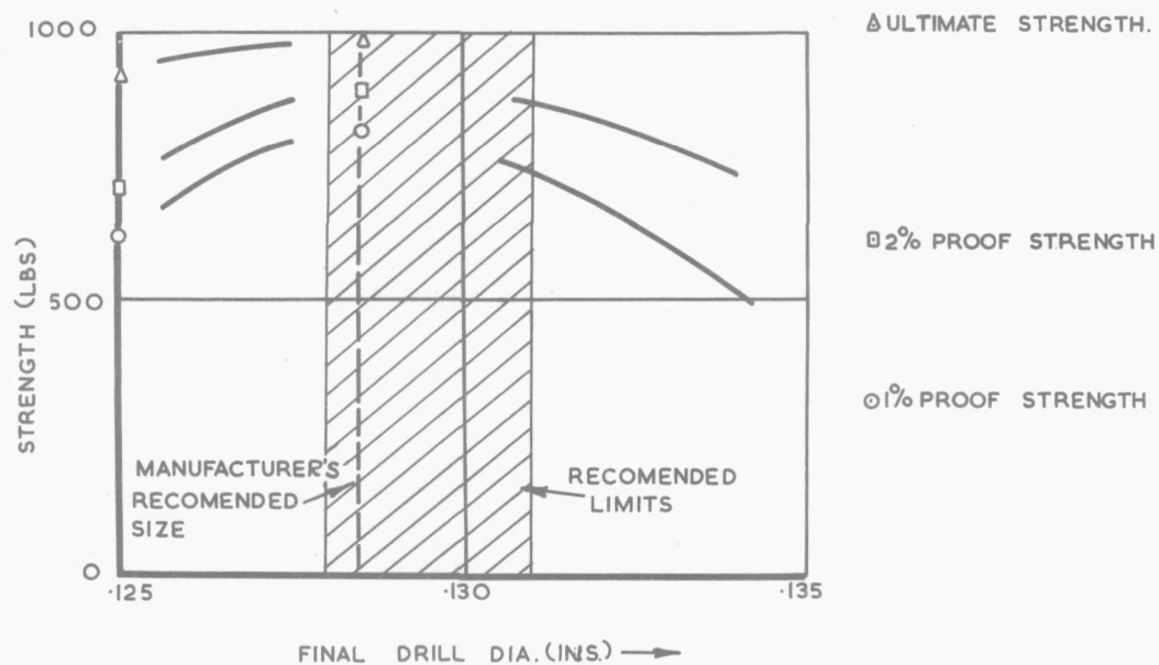
FIG.7 EFFECT OF FIT ON STRENGTH OF AVDEL RIVET LAP JOINT IN SINGLE SHEAR (2 : \frac{1}{8} DIA. RIVETS 14G. DTD546 B SHEET)
