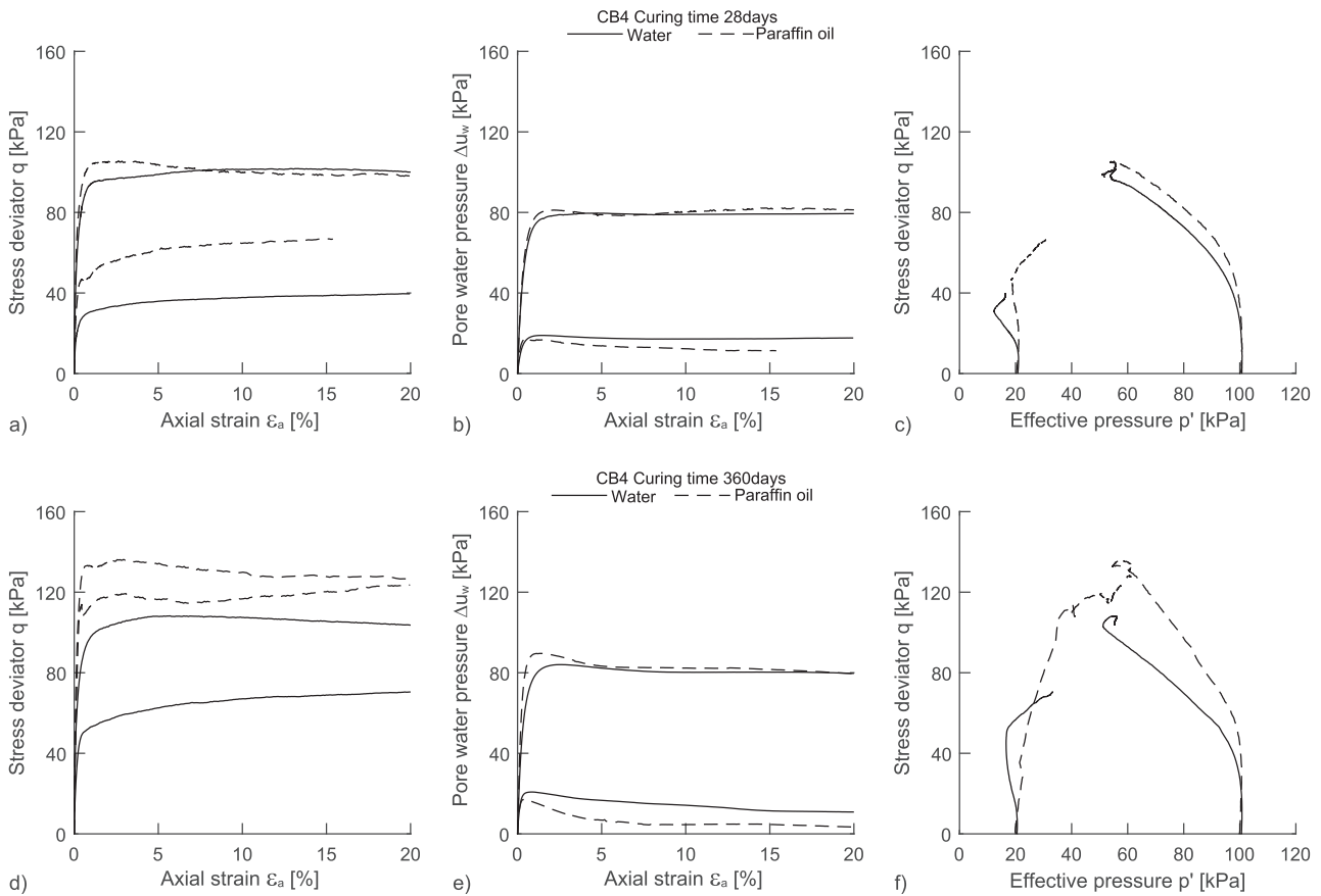
Fig. 10. Mixture CB4 triaxial tests ( p'_c = 20 and 100 kPa) results: a) q - \varepsilon_a plane curing 28 days, b) \Delta u_w - \varepsilon_a plane curing 28 days, c) q - p' plane curing 28 days, d) q - \varepsilon_a plane curing 360 days, e) \Delta u_w - \varepsilon_a plane curing 360 days and f) q - p' plane curing 360 days.
