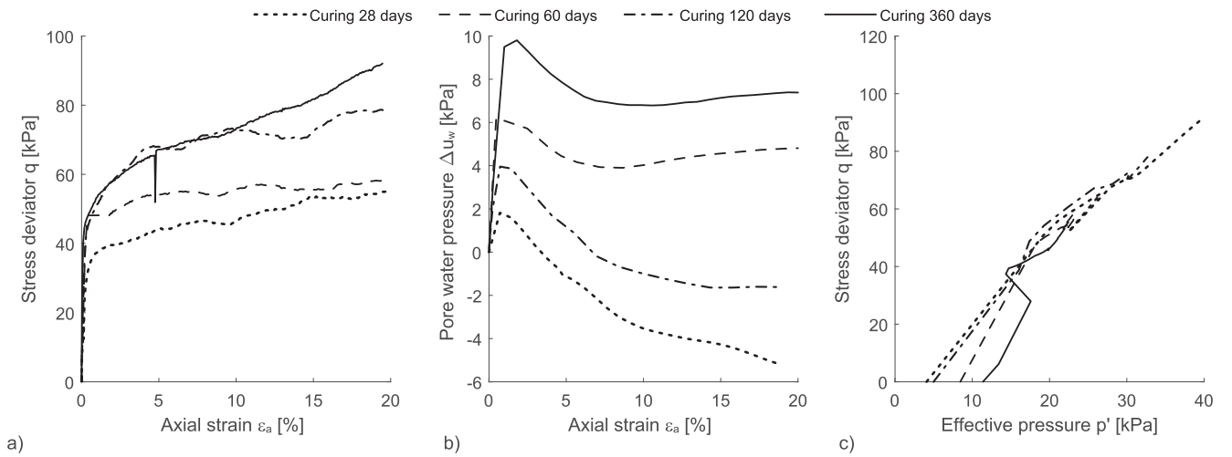
Fig. 18. Mixture CB4 undrained unconsolidated triaxial tests results (curing in water): a) q - \varepsilon_a plane, b) \Delta u_w - \varepsilon_a plane and c) q - p' plane.
