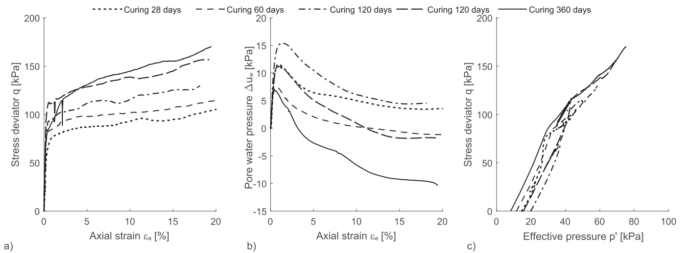
Fig. 19. Mixture CB5 undrained unconsolidated triaxial tests results (curing in water): a) q - \varepsilon_a plane, b) \Delta u_w - \varepsilon_a plane and c) q - p' plane.
