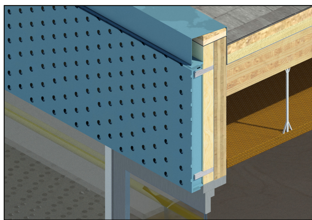
Rooftop
