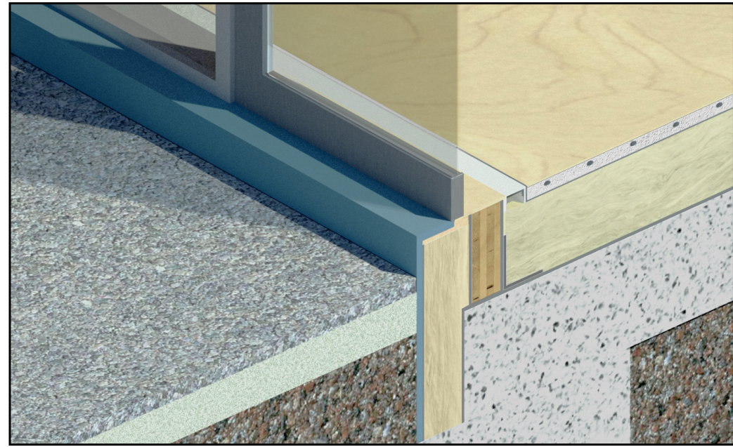
Foundation
