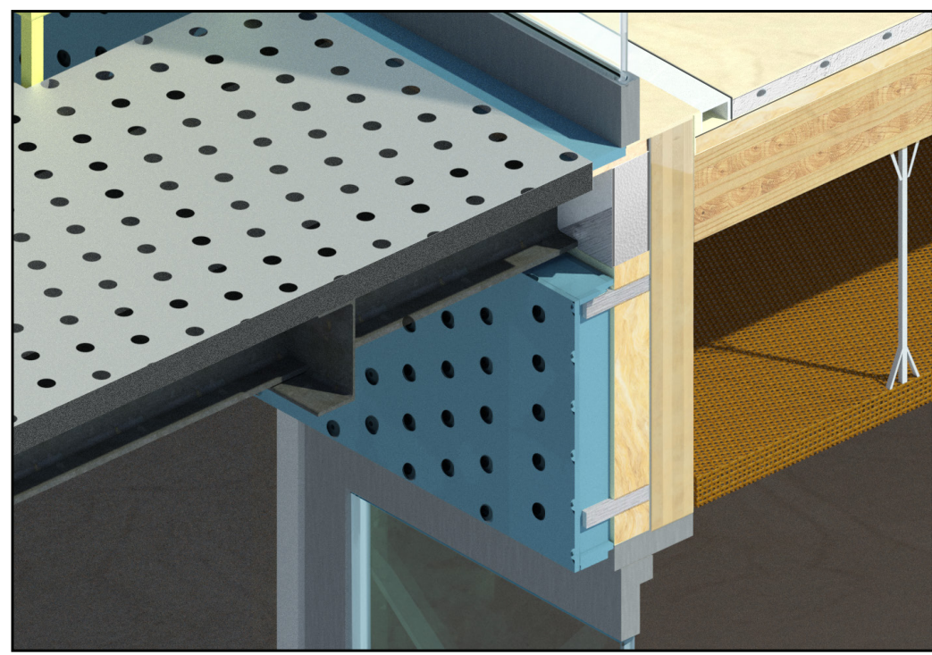
Steel gallery-to-wall
