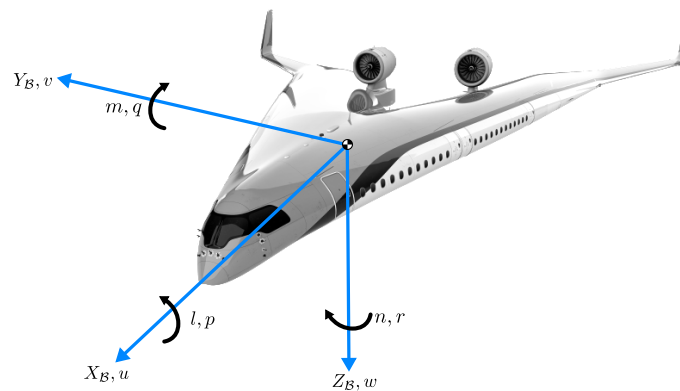
Fig. 2 Aircraft body axes and conventions. Adapted from [2]
