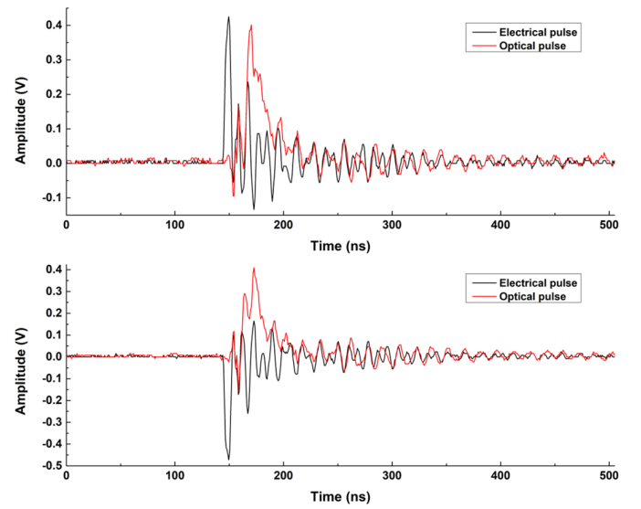
Fig. 7. Unipolar optical pulses and bipolar electrical pulses of a PD.
