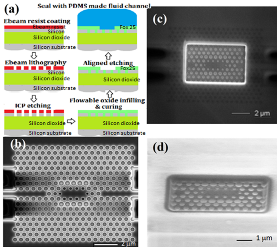
FIG. 3. (a) A flowchart of planarized-sensor-fabrication. (b) A scanning electron microscope (SEM) image of the photonic crystal after SF 6 and O 2 dry-etching. (c), (d) SEM images of the sensor with a carefully opened access on the cured Fox-25 protection layer. Fox-25 has been infiltrated in the holes and on the top, and made the surface of the sensor flat. The liquid-access was opened by aligned etching which stopped at the top surface of the silicon slab. Therefore the holes in this area were still filled with Fox-25.
