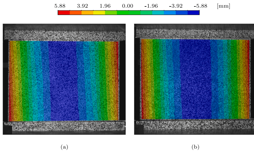
Fig. 15. Out-of-plane imperfections: (a) panel 1; (b) panel 2.
