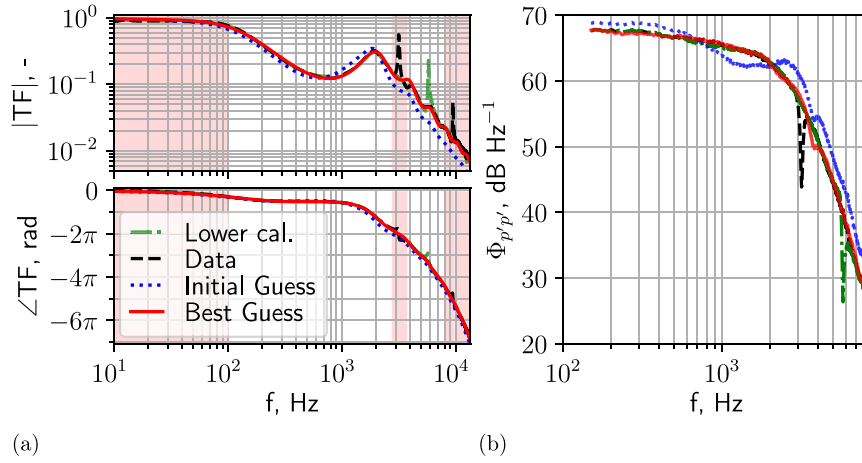
Fig. 16. RMP TF and WPS of a ZPG TBL flow. The 'Lower cal.' TF is acquired with a different calibrator side branch (Section 3.1) and is presented for comparison to the model fit. (a) RMP TF_{\text{ref} \rightarrow \text{RMP}} data and W model fit on 'Data'. The red-tinted regions denote band-removed frequency bands; (b) WPS acquired with RMP with an outer flow velocity of U_e = 19.7 \text{ m s}^{-1} .
