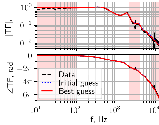
Fig. 15. RMP TF_{\text{ref} \rightarrow \text{RMP}} calibration data, which are not affected by the 'extra line-cavity element', and W model fit. The red-tinted regions denote band-removed frequency bands.
