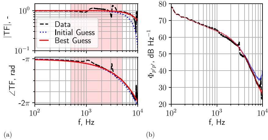
Fig. 10. Pinhole electret TF, and WPS data of a ZPG TBL flow. (a) TF_{\text{ref}} - \text{pin} calibration data and W model fit. The red-tinted regions denote band-removed frequency bands; (b) WPS for U_{\infty} = 19.7 \text{ m s}^{-1} .
