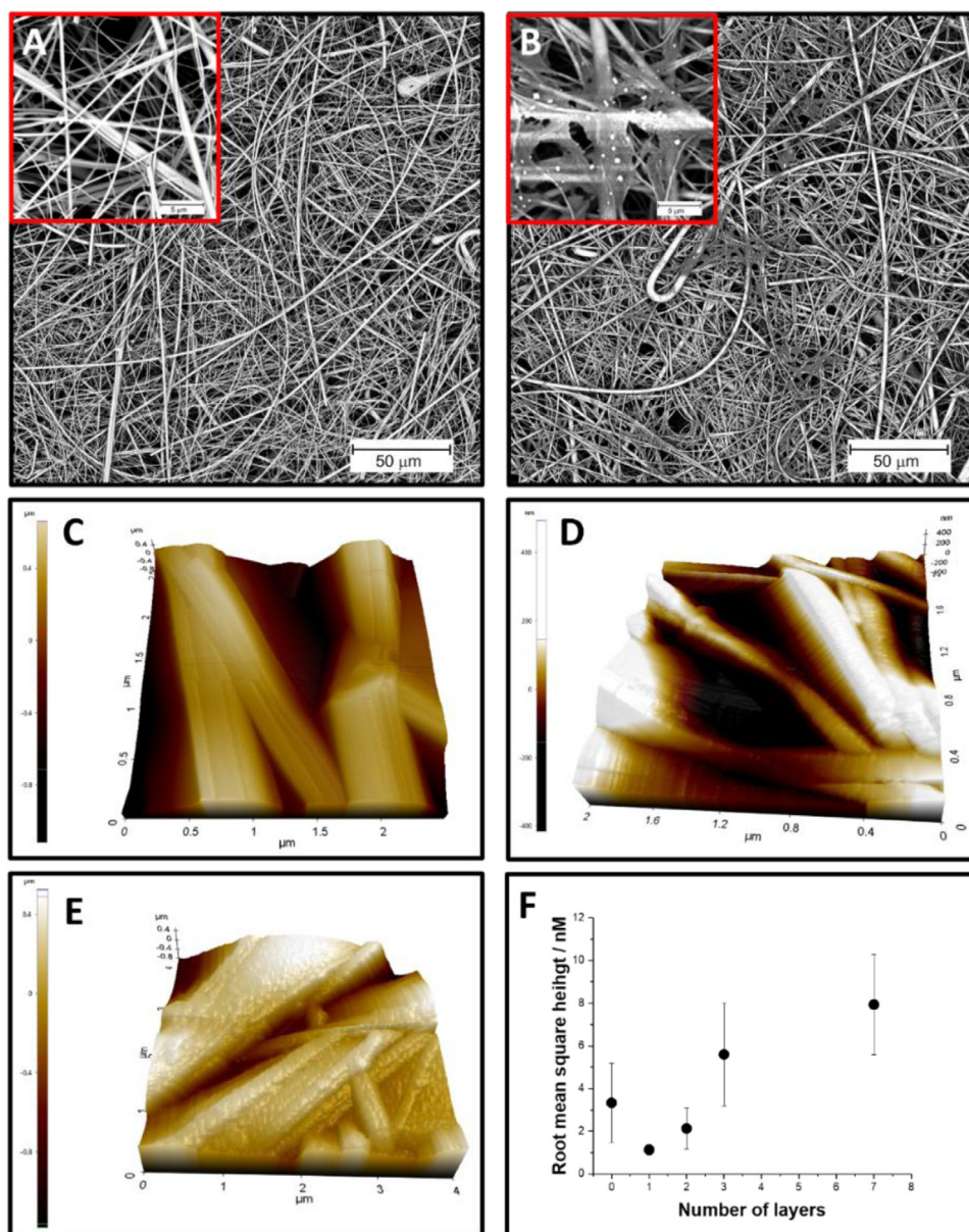
Fig. 7. A and B are the SEM micrographics recorded for the fiberglass membrane before and after modification with PEI(PSS/PHMG) 3 multilayer, respectively. Insets show the magnification. AFM topological images showing unmodified glass fibers ( C ), glass fibers modified with PEI(PSS/PHMG) 1 ( D ), and PEI(PSS/PHMG) 3 ( E ) are given as the bottom panel. F is the root mean square height calculated as an average from three positions as a function of polyelectrolyte layer thickness. The number of layers equal to zero represents the unmodified fiberglass membrane.
