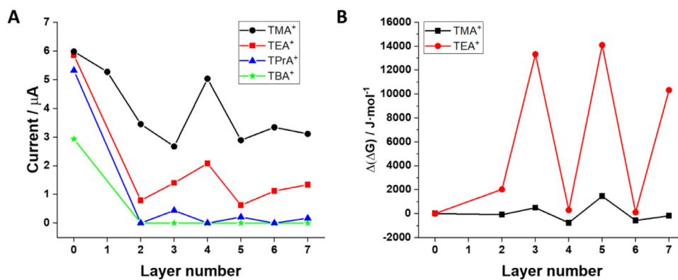
Fig. 9. A – Positive peak current values for four studied quaternary ammonium cations (see the corresponding legend) as a function of the layer thickness. Prepared based on Fig. S16 – S19. B – Change in the free Gibbs energy (Eq. (3)) of the ion transfer reaction for TMA + and TEA + as a function of the layer thickness. Prepared based on Fig. S16 and S17.
