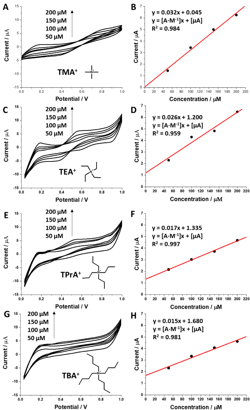
Fig. 5. Series of ion transfer voltammograms (and corresponding calibration curves – right column) recorded for a family of quaternary ammonium cations at the liquid-liquid interface supported with unmodified glass fiber membrane. The studied concentration equal to 50; 100; 150 and 200 \mu\text{M} . A and B – TMA + Cl - ; C and D – TEA + Cl - ; E and F – TPrA + Cl - ; G and H – TBA + Cl - . The scan rate was 20 mV·s -1 .
