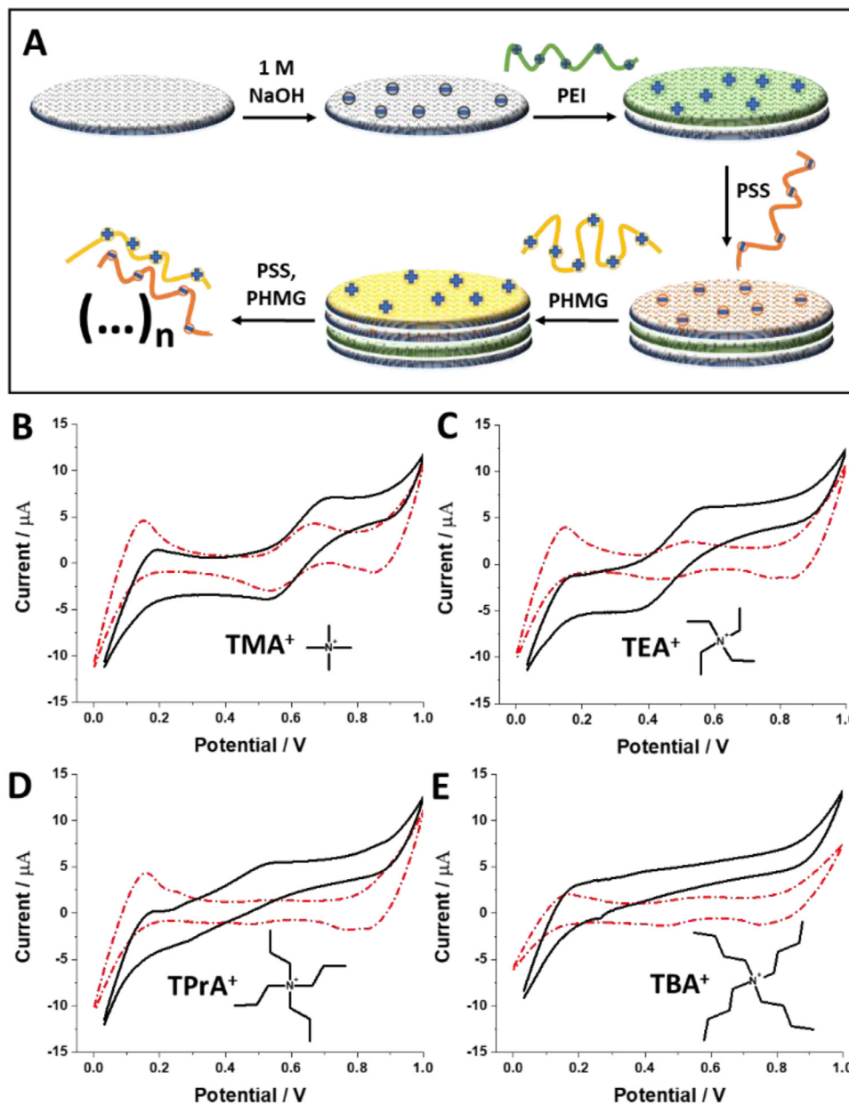
Fig. 8. A – schematic and simplified representation of the polyelectrolyte multilayer growing at the surface of the fiberglass membrane. B, C, D, and E are the ITVs recorded before (solid, black line) and after (red, dash-dot lines) fiberglass membrane modification with PEI(PSS/PHMG) 3 for TMA + , TEA + , TPrA + and TBA + respectively. The concentration of each quaternary ammonium cation was set to 200 μM. Scan rate = 20 mV·s -1 .
