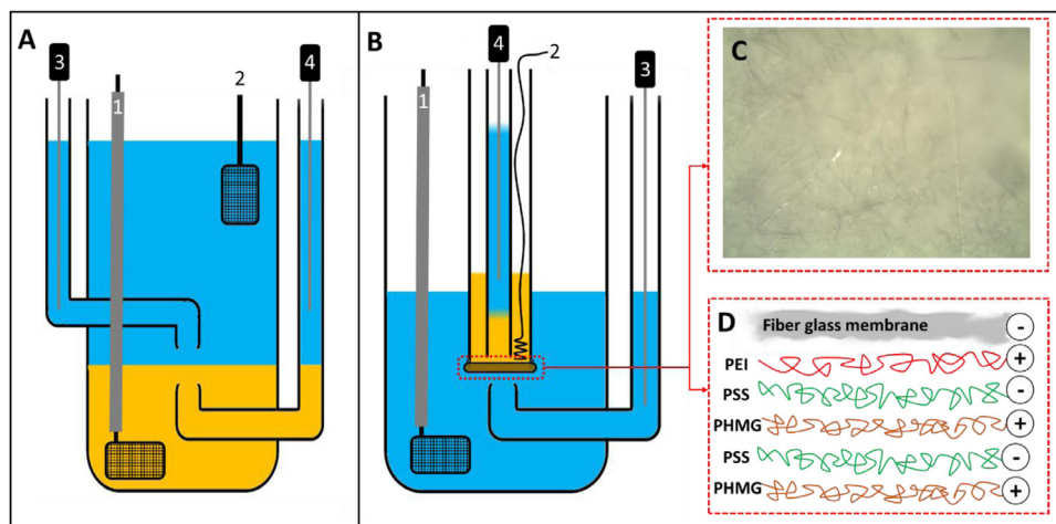
Fig. 1. A – the classical glass cell used to support macroscopic LLI; B – the glass cell used to study the modified and unmodified fiberglass membrane supported LLI; C – the optical microscopy photo of the unmodified glass fiber membrane; D – schematic representation of the fiberglass membrane modified with polyelectrolyte multilayer. 1 and 2 are the organic phase and the aqueous phase counter electrodes, respectively. 3 and 4 are the Ag/AgCl reference electrodes placed in both phases each. PEI - poly(ethyleneimine); PSS - polystyrene sulfonate; PHMG - polyhexamethylene guanidine.
