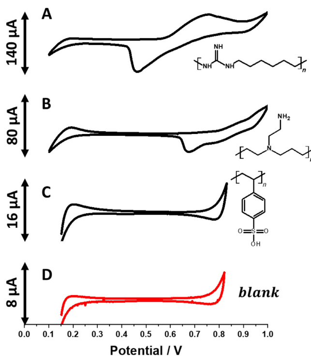
Fig. 2. Ion transfer voltammograms recorded for A – 50 μg/mL PHMG (aqueous phase: 10 mM NaCl); B – 50 μg/mL PEI (aqueous phase: 10 mM HCl in 10 mM NaCl); C – 50 μg/mL PSS (aqueous phase: 10 mM NaCl); D – blank voltammogram (aqueous phase: 10 mM NaCl). The organic phase was 5 mM BTTPATPBCl dissolved in 1,2-dichloroethane. Scan rate was 10 mV·s -1 . Structures of an uncharged polyelectrolyte are placed on the right from the corresponding voltammogram.
