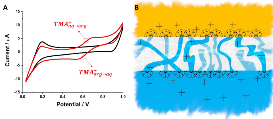
Fig. 4. A – ion transfer voltammograms recorded at the LLI supported with the unmodified fiberglass membrane in the presence (red curve) and the absence (black curve) of 150 μM TMA^+Cl^- initially dissolved in the aqueous phase. The scan rate was 20 mV·s -1 . B – schematic representation of the fiberglass membrane supporting LLI with the hemispherical diffusion zones established on the pores ingress from the aqueous and the organic phase side. (For interpretation of the references to color in this figure legend, the reader is referred to the web version of this article.)
