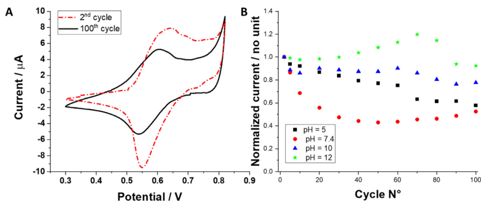
Fig. 3. A – the ion transfer voltammograms recorded in cell II, for PHMG = 20 μg/mL, for the 2 nd (red, dot-dash curve) and 100 th cycle (black, solid curve). B – forward signal peak currents normalized values recorded over 100 consecutive scans for pH equal to 5.0; 7.4; 10.0 and 12.0 (for the symbols refer to the legend available in the inset). (For interpretation of the references to color in this figure legend, the reader is referred to the web version of this article.)
