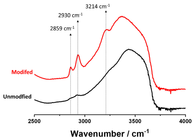
Fig. 6. Infra-red spectra recorded for unmodified (black, bottom curve) and polyelectrolyte multilayer modified (red, upper curve) membrane. Absorption bands of interest are indicated with arrows. Polyelectrolyte layer thickness – PEI(PSS-PHMG) 5 . (For interpretation of the references to color in this figure legend, the reader is referred to the web version of this article.)
