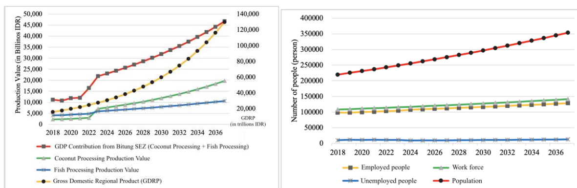
Figure 12 The economy module (left) and the social module (right) simulation results for business-as-usual scenario
