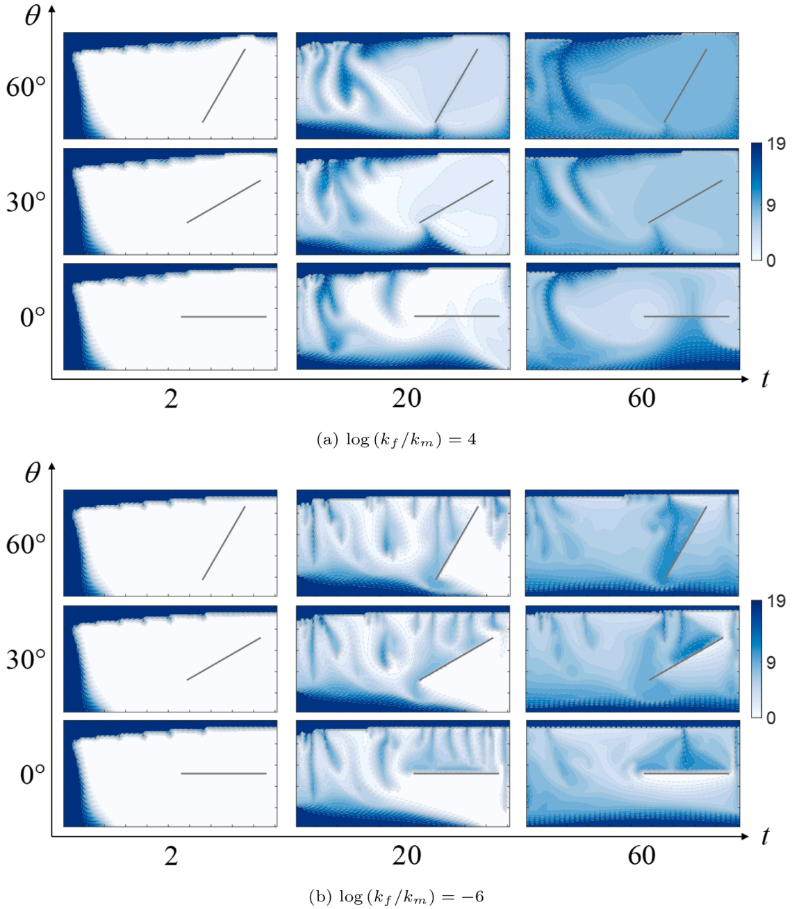
Fig. 10. Solution CO 2 -brine ratio profiles in cases of a fracture placed near the production well ( k_m = 8.0 \times 10^{-14} m 2 ).
