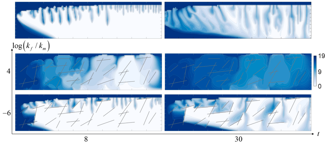
Fig. 20. Solution \text{CO}_2 -brine ratio profiles in case of fracture network ( k_m = 8.0 \times 10^{-14} \text{ m}^2 ). Results obtained from the base case (without fractures) are presented on top.
