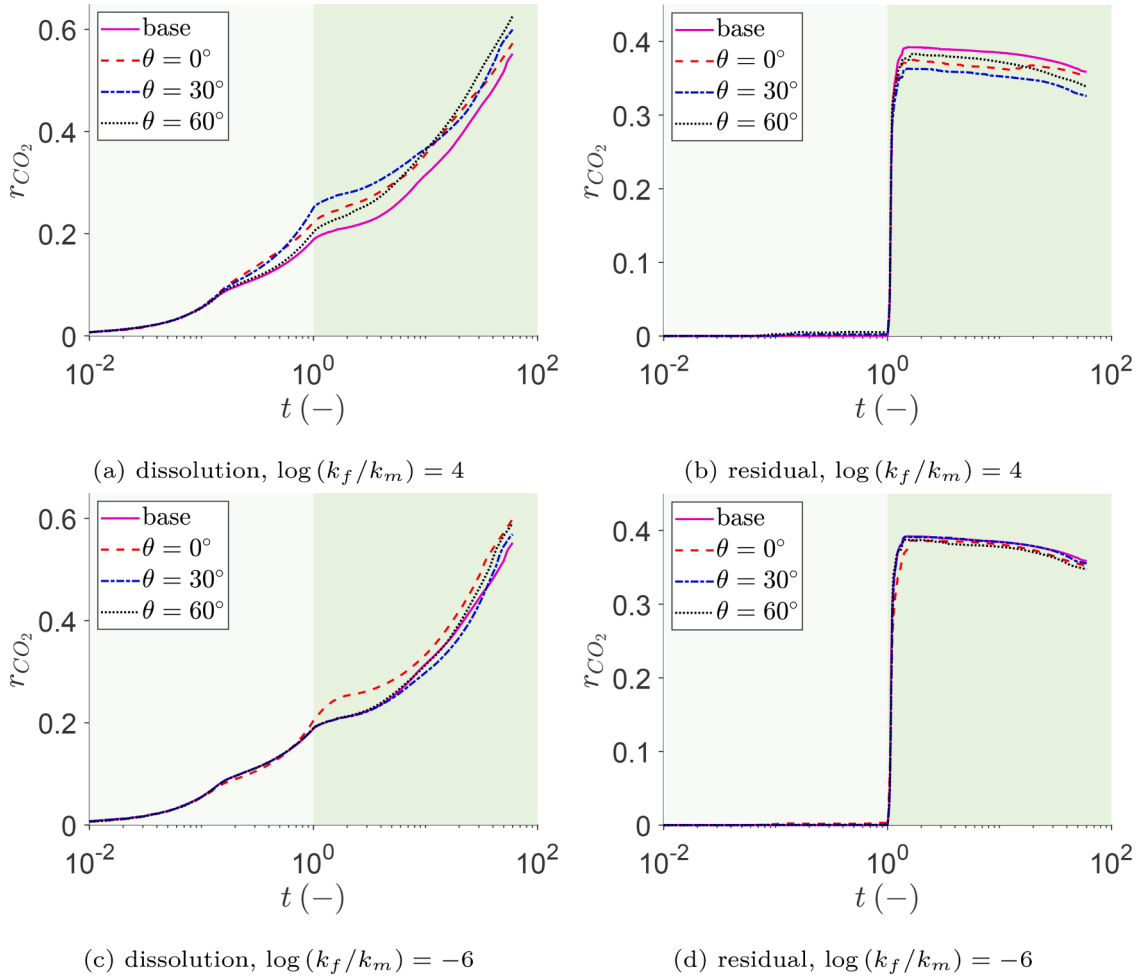
Fig. 5. Fraction of injected CO 2 trapped by different mechanisms in cases of a fracture placed near the injection well ( k_m = 8.0 \times 10^{-14} \text{ m}^2 ).
