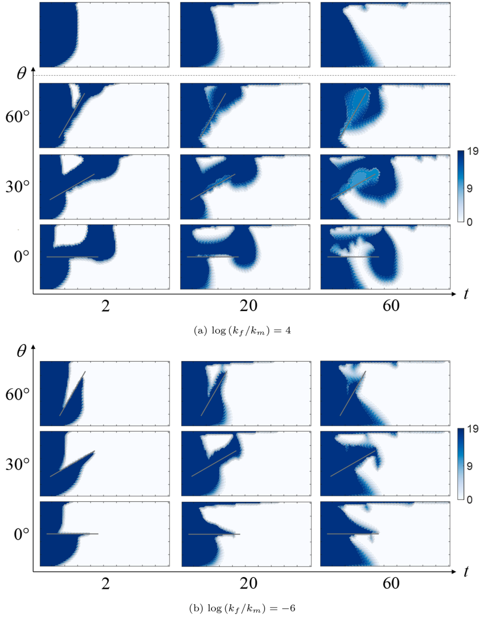
Fig. 14. Solution \text{CO}_2 -brine ratio profiles in cases of a fracture placed near the injection well ( k_m = 4.0 \times 10^{-15} \text{ m}^2 ). Results obtained from the base case (without fractures) are presented on top of the cases with \log(k_f/k_m) = 4 .
