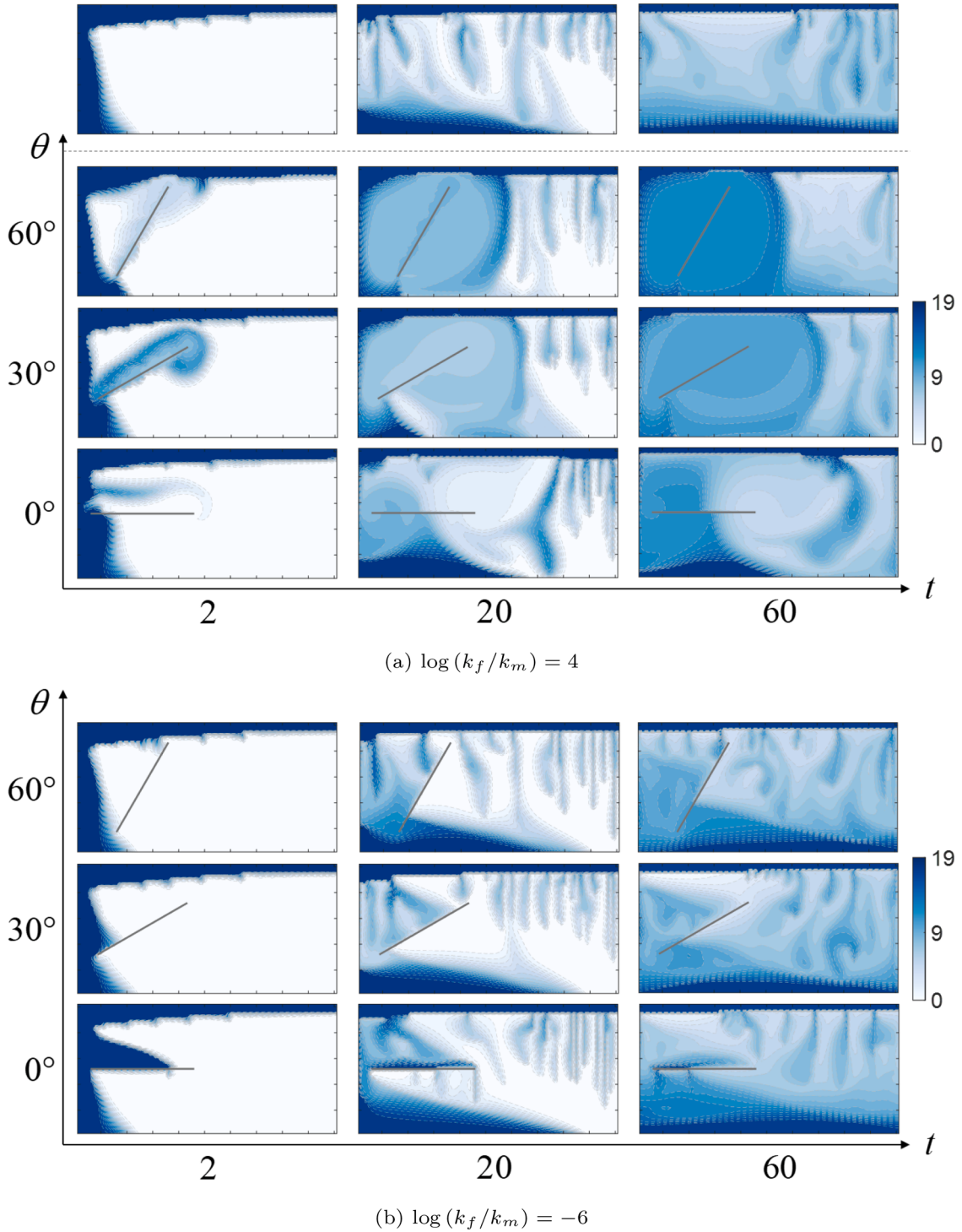
Fig. 7. Solution \text{CO}_2 -brine ratio profiles in cases of a fracture placed near the injection well ( k_m = 8.0 \times 10^{-14} \text{ m}^2 ). Results obtained from the base case (without fractures) are presented on top of the cases with \log(k_f/k_m) = 4 .
