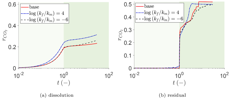
Fig. 21. Fraction of injected \text{CO}_2 trapped by different mechanisms in the case of a fracture network ( k_m = 4.0 \times 10^{-15} \text{ m}^2 ).
