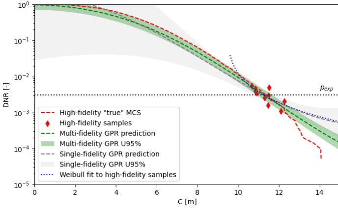
FIGURE 9: Results for sample option SampPexp , with Meas-Noise . Screening + single- / multi-fidelity GPR / Weibull fit results.
