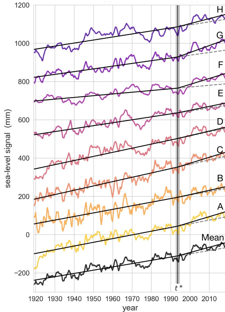
Figure 3. The extracted monthly sea-level signal (colored curves) and the fitted PWLF (black lines) from the tide gauges analyzed in this study. An arbitrary offset is added to the individual time series for better visualization. The locations of the tide gauges are shown in the inset. The detected breakpoint t^* is shown with a vertical line and the 95% confidence interval obtained with the Markov Chain Monte Carlo analysis is shaded (August 1993 \pm 11 months).
