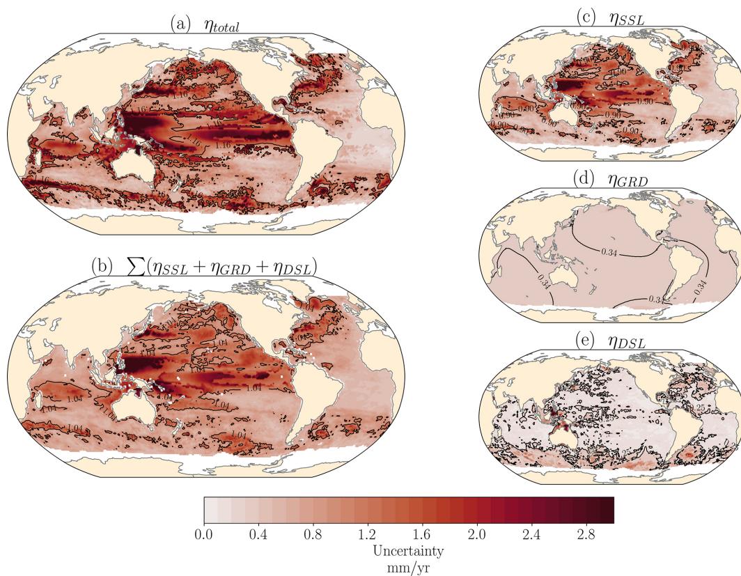
Figure A2. Uncertainties of the regional sea-level trends (Fig. 1) for 1993–2016 (mm yr -1 ) for (a) altimetry, (b) sum of sea-level components, (c) full-depth steric, (d) GRD effect, and (e) dynamic sea-level change. The black contour line indicates global mean sea-level change.
