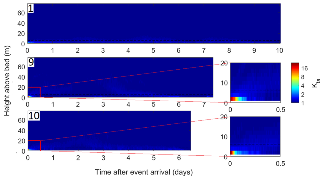
Figure 4. Derived calibration constant anomaly ( K_{ta} ) values for Events (top) 1, (middle) 9, and (bottom) 10. Details of the flow front are shown in more detail. Dashed lines show the potential extent of the near-bed sidelobe region. K_{ta} values should be constant for the ADCP. Variations in K_{ta} thus highlight where flow may be coarser-grained or higher-concentration than in the single grain size distribution model.
