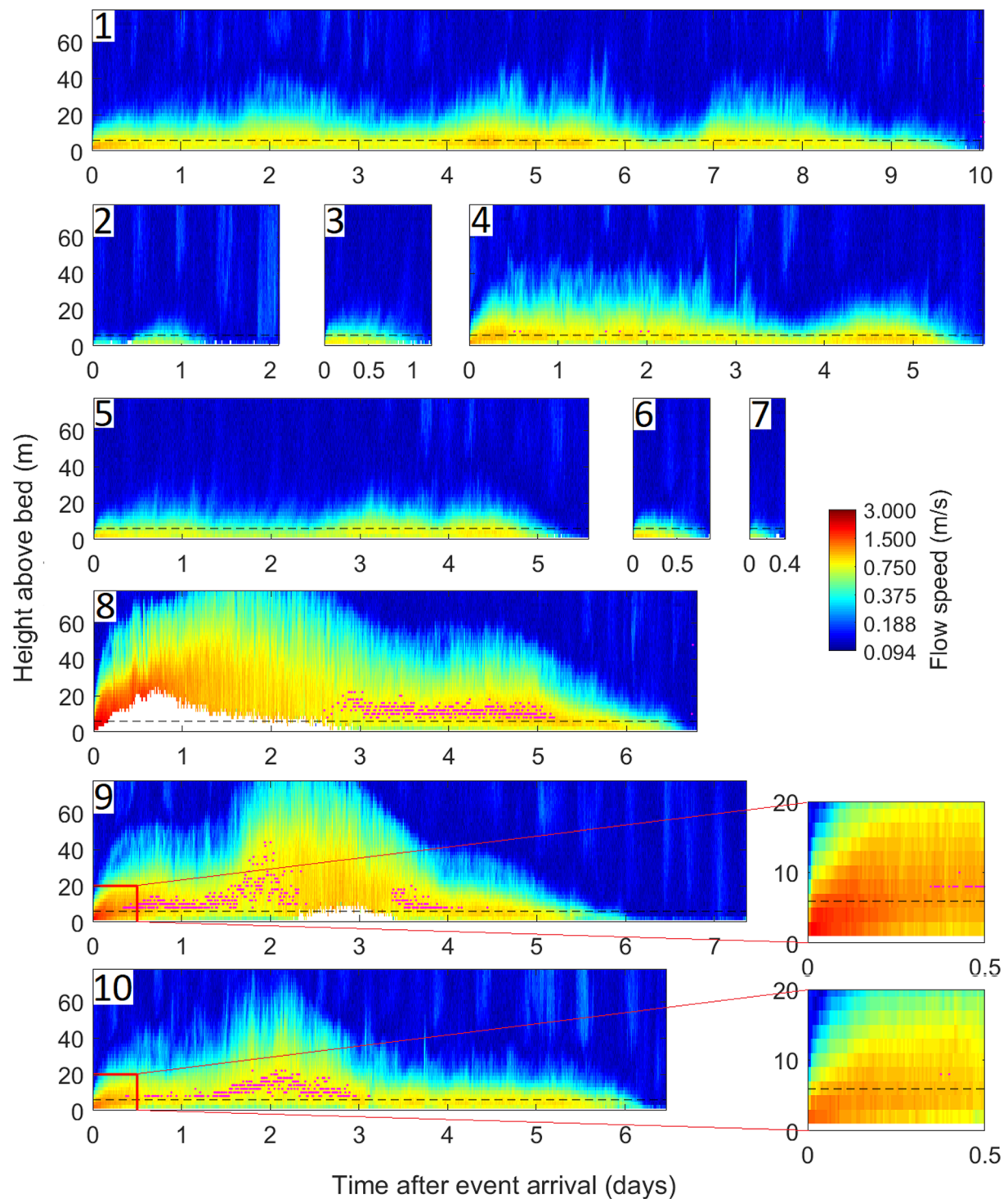
Figure 6. Velocity structure of 10 turbidity currents in the Congo Canyon. Velocities measured every 5 s by the 300 kHz ADCP and averaged over 500 s intervals. Details of flow front shown for Events 9 and 10. Dashed lines show height that is 6% of distance from bed to ADCP, where side lobe interference can occur, if sediment concentrations are not sufficiently high. Purple dots show height of velocity maximum, when it can be identified confidently (i.e., it is above sidelobe interference region, and there is no major data loss due to signal-to-noise issues). Azpiroz-Zabala et al. (2017) provide a detailed analysis of Event 9.
