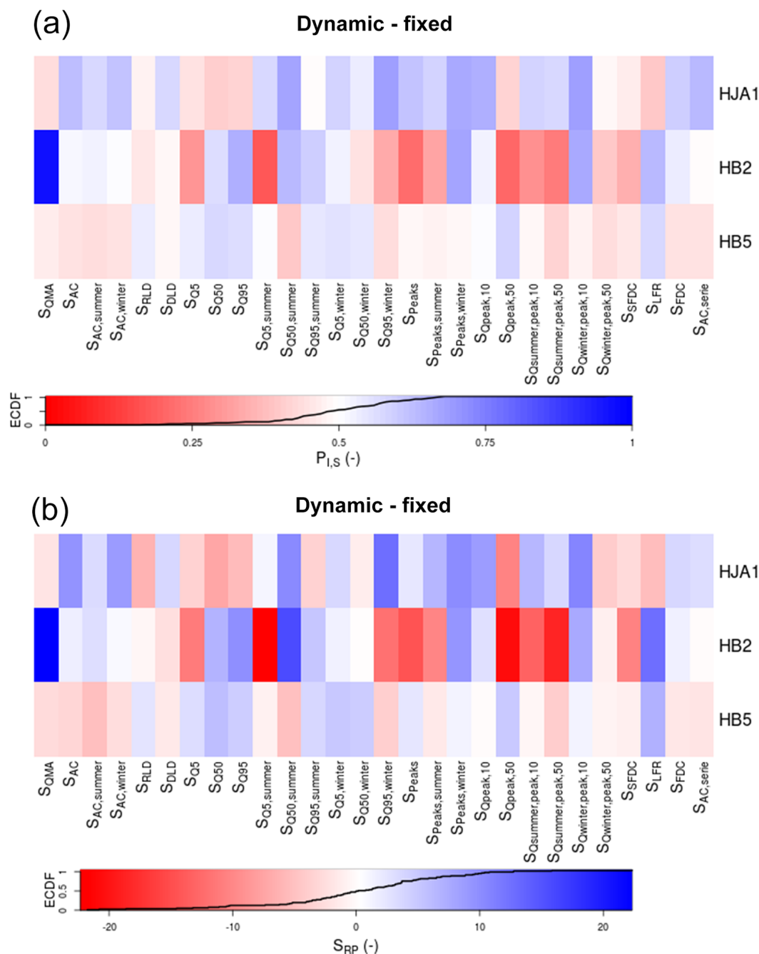
Figure 9. Signature comparison between a time-dynamic and time-invariant formulation of root-zone storage capacity in the FLEX model with (a) probabilities of improvement and (b) Ranked Probability Score for 28 hydrological signatures for HJ Andrews WS1 (HJA1), Hubbard Brook WS2 (HB2) and Hubbard Brook WS5 (HB5). High values are shown in blue, whereas a low values are shown in red.
