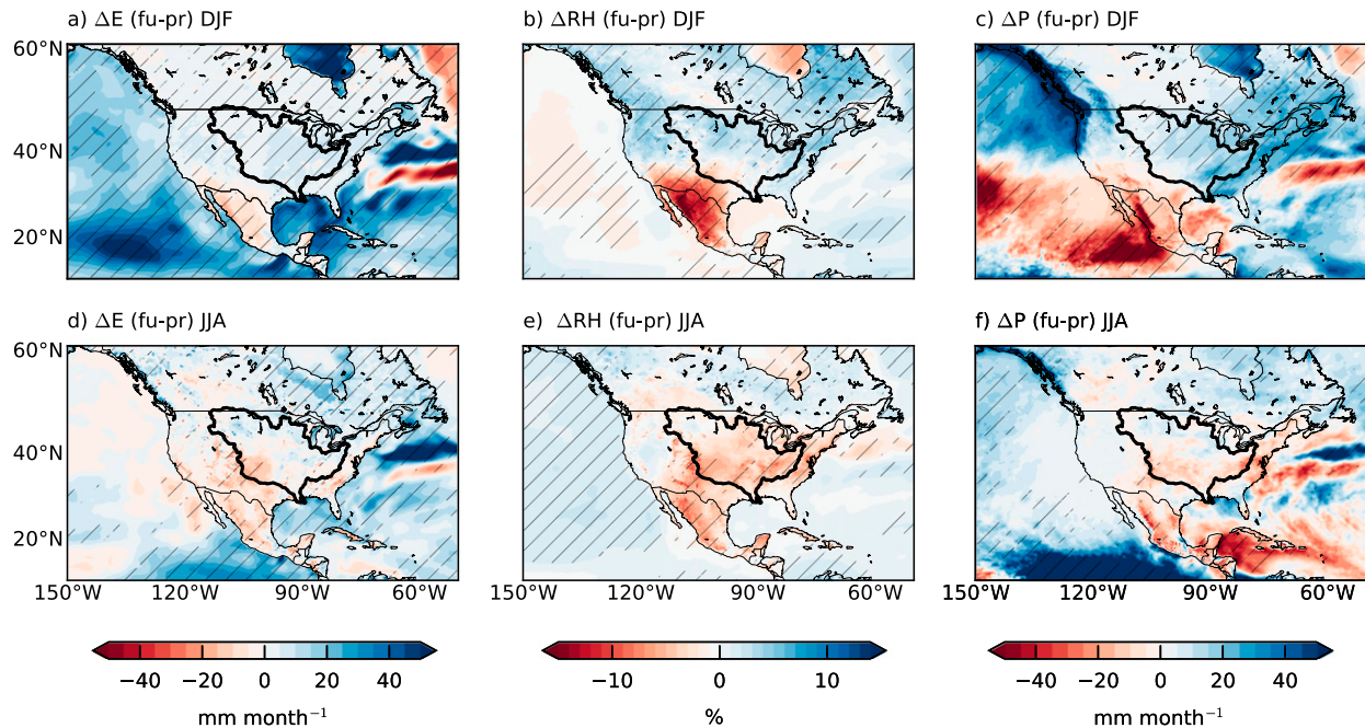
FIG. 3. Spatial patterns of the change in EC-Earth RCP4.5 (a),(d) evaporation \Delta E (future – present; \text{mm month}^{-1} ), (b),(e) relative humidity \Delta RH (future – present; %), and (c),(f) precipitation \Delta P (future – present; \text{mm month}^{-1} ) for (top) DJF and (bottom) JJA. Significant differences are indicated with hatching.
