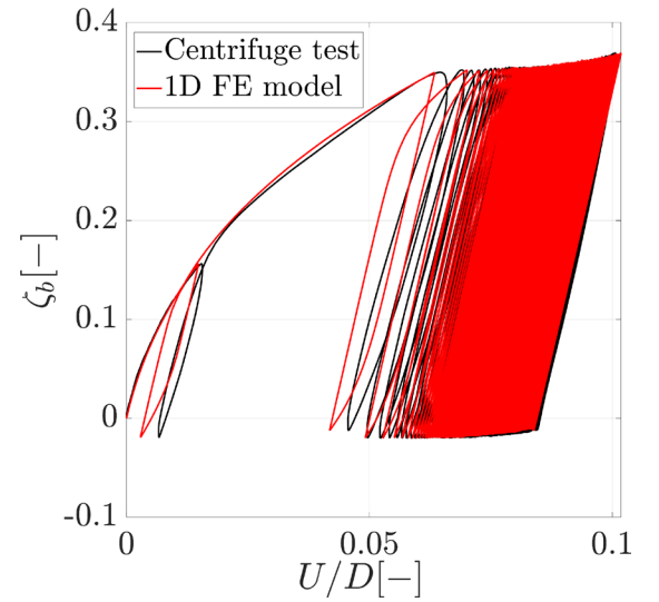
Figure 6a. Normalized load ( \zeta_b = F/F_f ) versus lateral normalized displacement trends from centrifuge measurements and numerical simulations at 8.5m above the soil surface
