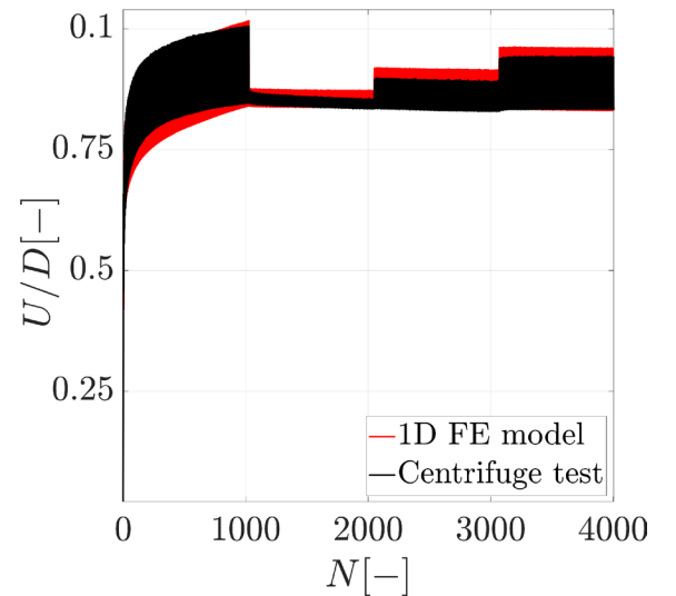
Figure 6b. Normalized displacement trends from centrifuge measurements and numerical simulations at 8.5m above the soil surface
