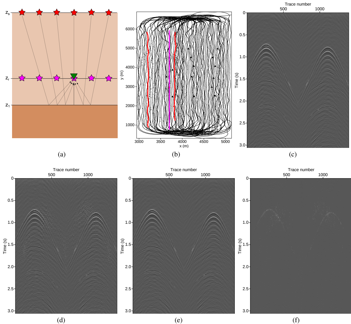
Figure 1: (a) Schematic representation of single-sided focusing, red original sources, magenta virtual sources at the focusing grid. The dotted traveltime is removed by the focal operator; (b) Acquisition plan for the field data, red : chosen node and sources, magenta : focusing grid; (c) Unblended data; (d) Pseudodeblended data; (e) Deblended data; (f) Deblending error, multiplied by 5.
