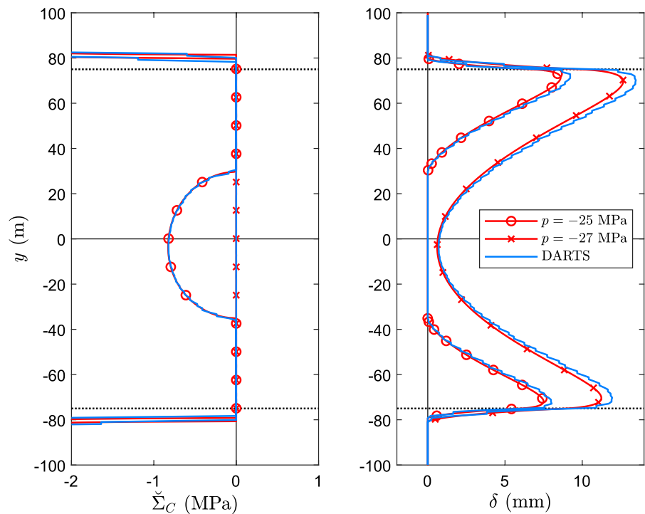
Fig. 10 Left: post-slip Coulomb stresses \tilde{\Sigma}_C . Right: the corresponding slip \delta . Simulation domain width W = 18,000 m
