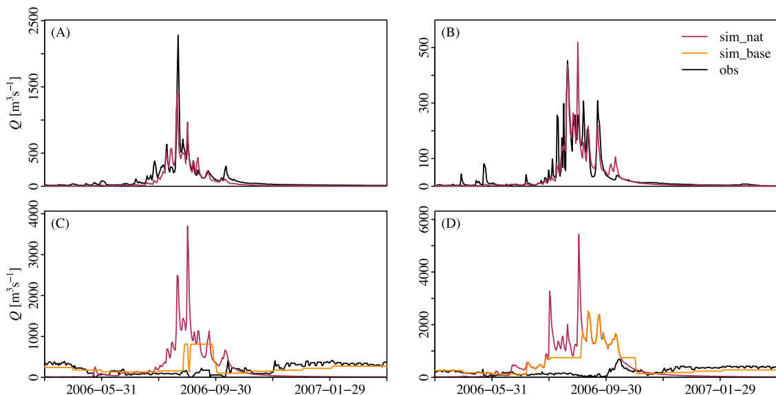
Fig. 2. Simulated and observed daily streamflows for the Nan_natural (A), Yom_natural (B), Sirikit (C) and Bhumibol (D) catchments in the wet year (2006). The streamflow in the naturalized scenario (sim_nat) is shown in red lines, the baseline operation scenario (sim_base) in orange lines and the observations (obs) in black lines. Since the hydrographs in the dry year (2013) show similar flow patterns, they are not included here.
