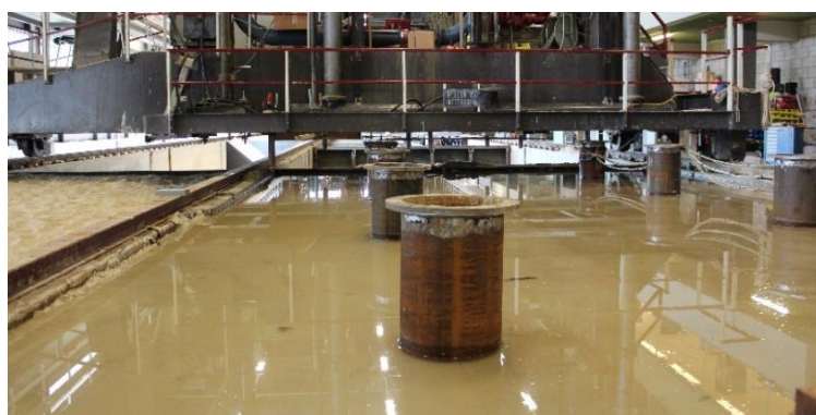
Figure 1: Water-Soil Flume at Deltares, with scaled piles installed in sand.
