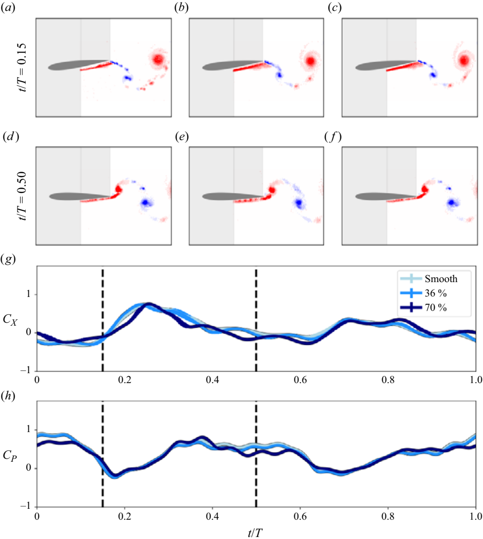
Figure 2. PIV results for Re = 28\,000 : t/T = 0.15 (a–c) and t/T = 0.50 (d–f) for the smooth (a,d), 36 % (b,e) and 70 % (c,f). Instantaneous C_X (g) and instantaneous C_P (h). Panels (g,h) contain confidence intervals calculated as CI = 4.6\sigma/\sqrt{N} .
