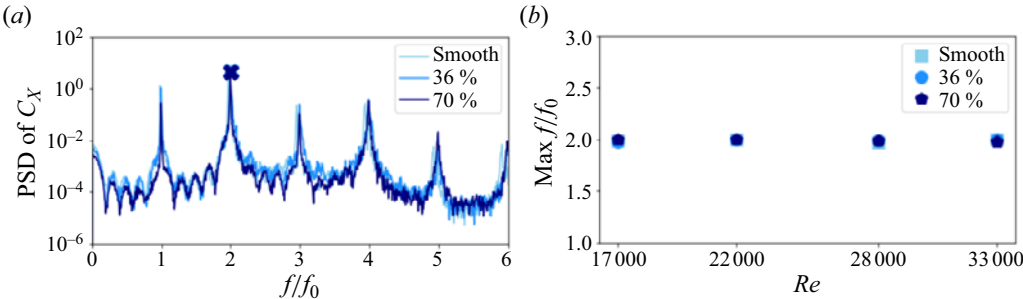
Figure 3. (a) Power spectral density analysis of the instantaneous C_X at Re = 28\,000 . The cross indicates the location of the peak for each case. (b) Peak frequency across the Re values considered. A value of 2 denotes that the thrust force signal f is equal to twice the input pitching frequency f_0 .
