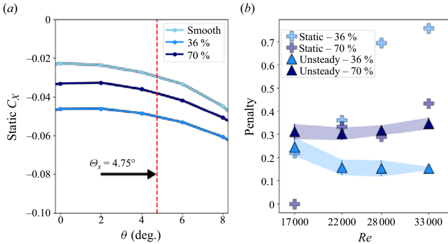
Figure 6. (a) Static C_X vs angle of attack \Theta measured using static foils at Re = 28\,000 . Smooth foil is presented in light blue, 36 % in medium blue and 70 % in dark blue. The red dashed line indicates the \theta used to compare with the unsteady regime, defined as \theta_s = 4.75^\circ . (b) Thrust and drag penalty due to roughness for both the flapping (triangles) and static results (crosses) for the 36 % case (medium blue) and the 70 % case (dark blue). The shadow region introduces the confidence intervals calculated as CI = 4.6\sigma/\sqrt{N} .
