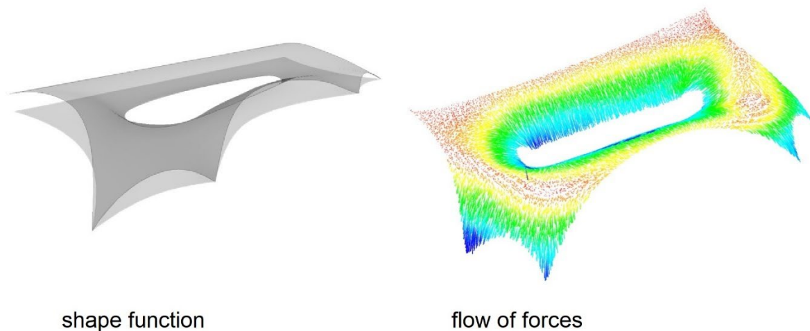
Figure 62 “rain shower” , load distribution of shell [images 52]
