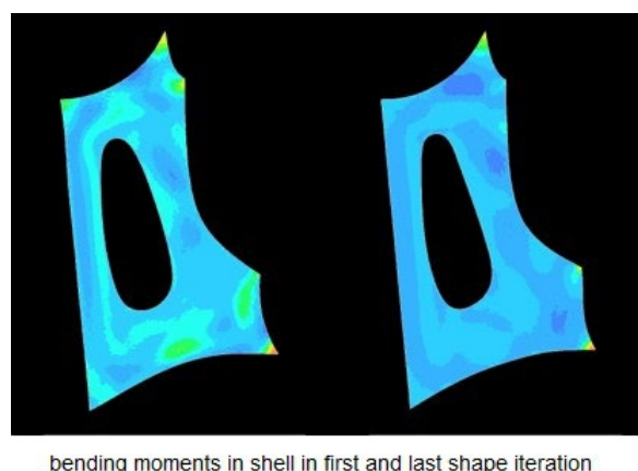
Figure 63 FEM calculation shell, top view [images 52]
