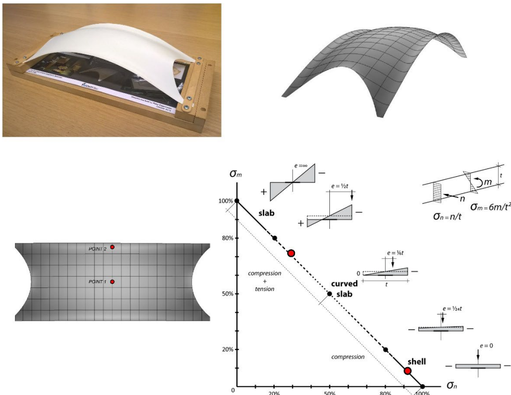
Figure 60 analysing shell Heinz Isler [images 106]
