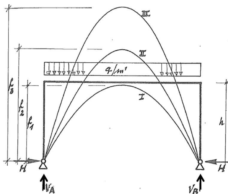
statically indeterminate
