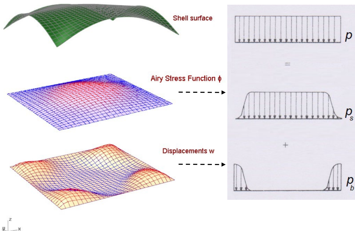
Figure 67 load carried by axial forces or bending moments [images left 108 and right 110]
