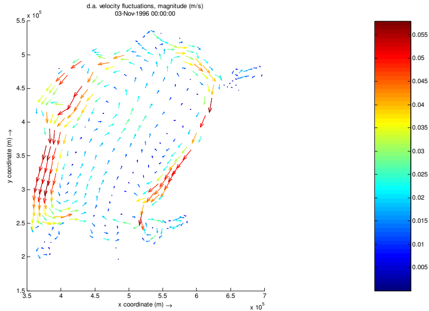
Figure 5.6: Hydrodynamic simulation under the October-December on 03 November 1996
