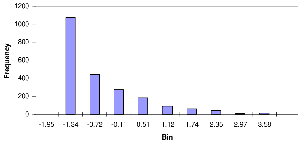
Figure 3.7 Histogram of bed shear stress after transformation
