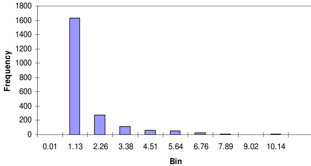
Figure 3.6 Histogram of bed shear stress before transformation
