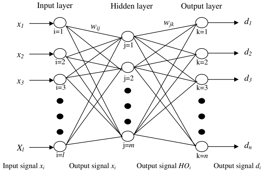
Figure 4.1 shows a schematisation of an MLP network topology
