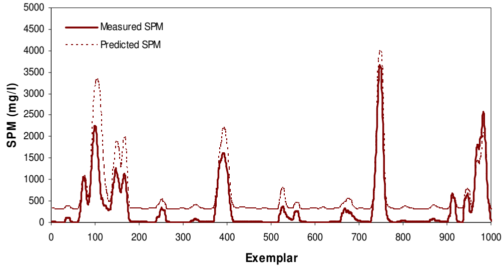
Figure 3.8 plot of desired and predicted SPM using untransformed data
