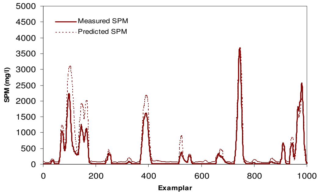
Figure 3.9 Plot of desired and predicted SPM using transformed data
