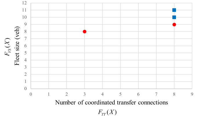
Fig. 5. Trade-off between the number of coordinated transfer connections and the required minimal fleet size.
