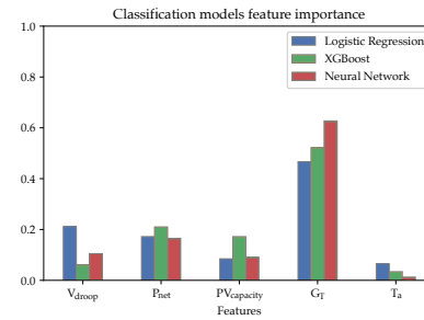
Fig. 8. Feature importance for the different classification models.
