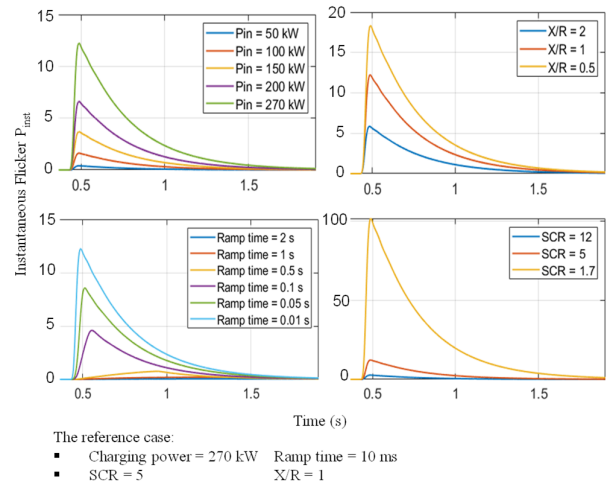
Fig. 3. The impact of influential factors on flicker.
