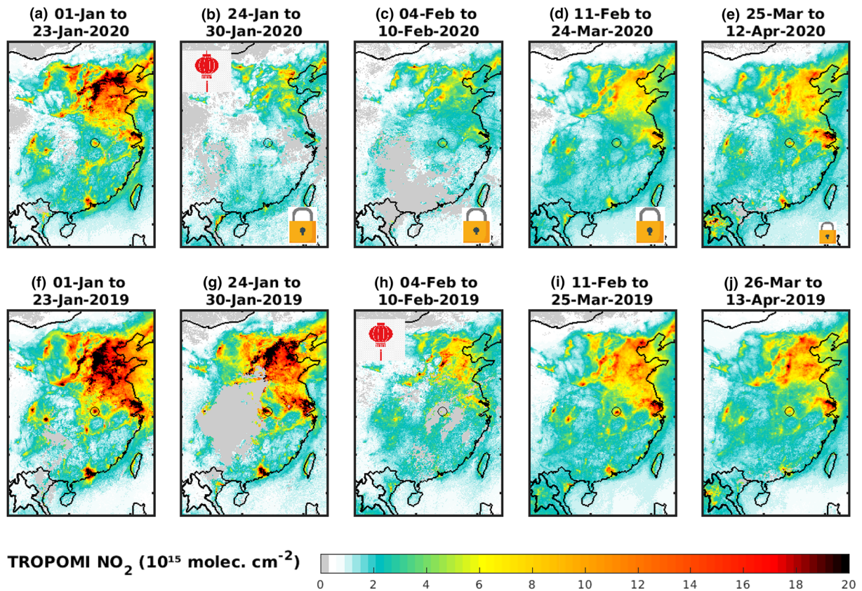
Figure 1. TROPOMI \text{NO}_2 columns over China (a) before and (b–e) after the lockdowns (shown by padlocks) due to Covid-19. For comparison, columns over the same time periods are shown for 2019. The week of Chinese new-year holiday is indicated by the red lantern shown inset panels (b) and (h). The New Year holiday covers 4–10 February in 2019 and 24–30 January in 2020 (exceptionally extended to 2 February because of Covid-19). Partial loosening of the restrictions is suggested by the smaller padlock in panel (e). Gray areas indicate no valid data.
