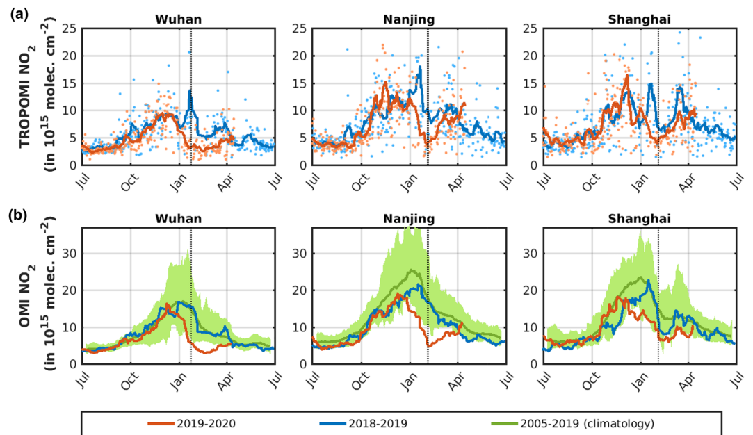
Figure 2. Spaceborne \text{NO}_2 columns within a 100 km radius around Wuhan, Nanjing, and Shanghai (blue symbols for 2018–2019 and red symbols for 2019–2020) and 14-day running averages (colored lines). (a) TROPOMI. (b) OMI, including climatological columns (2005–2019) and their range (green).
