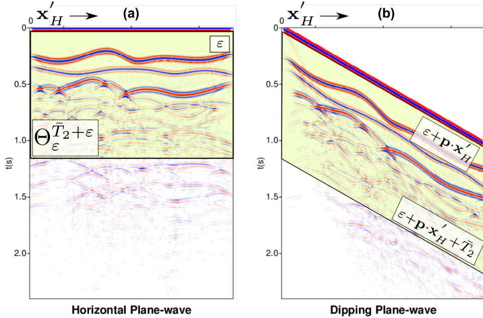
Figure 1 The shaded green areas show the support of representative muting operators for horizontal ( \Theta_{\varepsilon}^{\bar{T}_2 + \varepsilon} in (a)) and dipping ( \Theta_{\varepsilon + \mathbf{p} \cdot \mathbf{x}'_H}^{\varepsilon + \bar{T}_2 + \mathbf{p} \cdot \mathbf{x}'_H} in (b)) plane-wave sources (the corresponding data are shown in the background).
