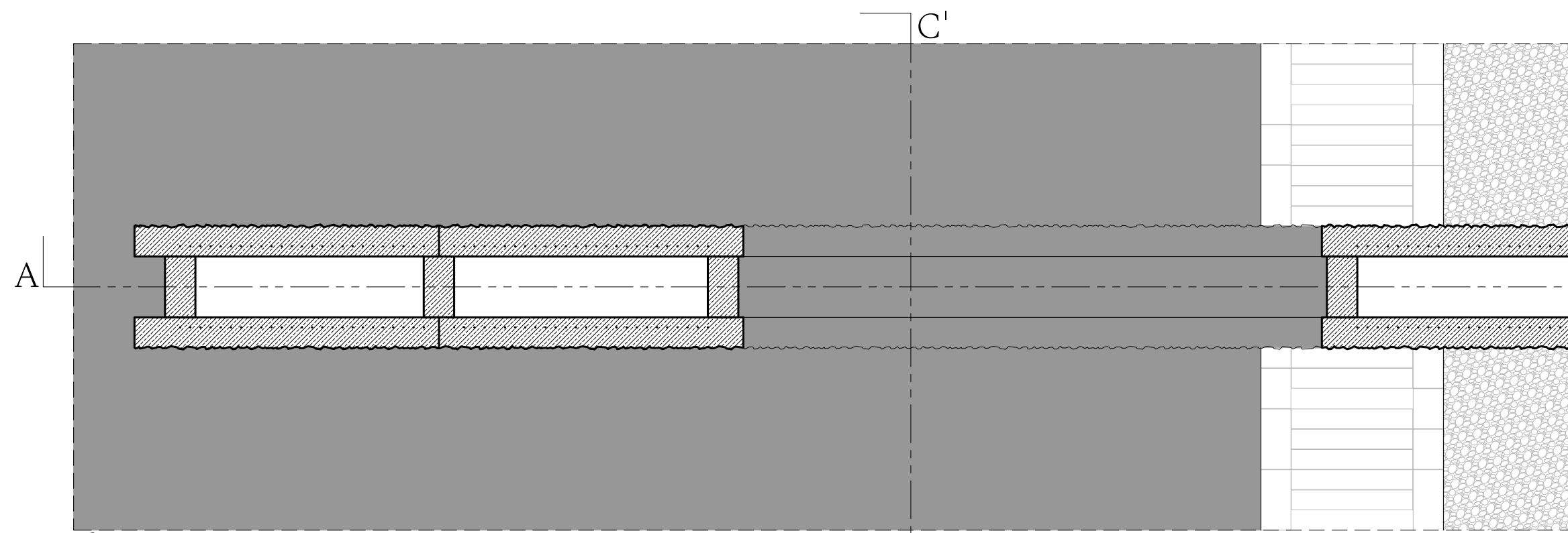
plan
