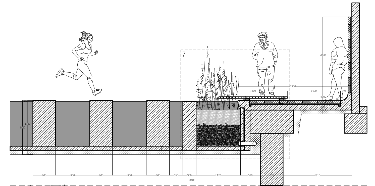
section CC'
