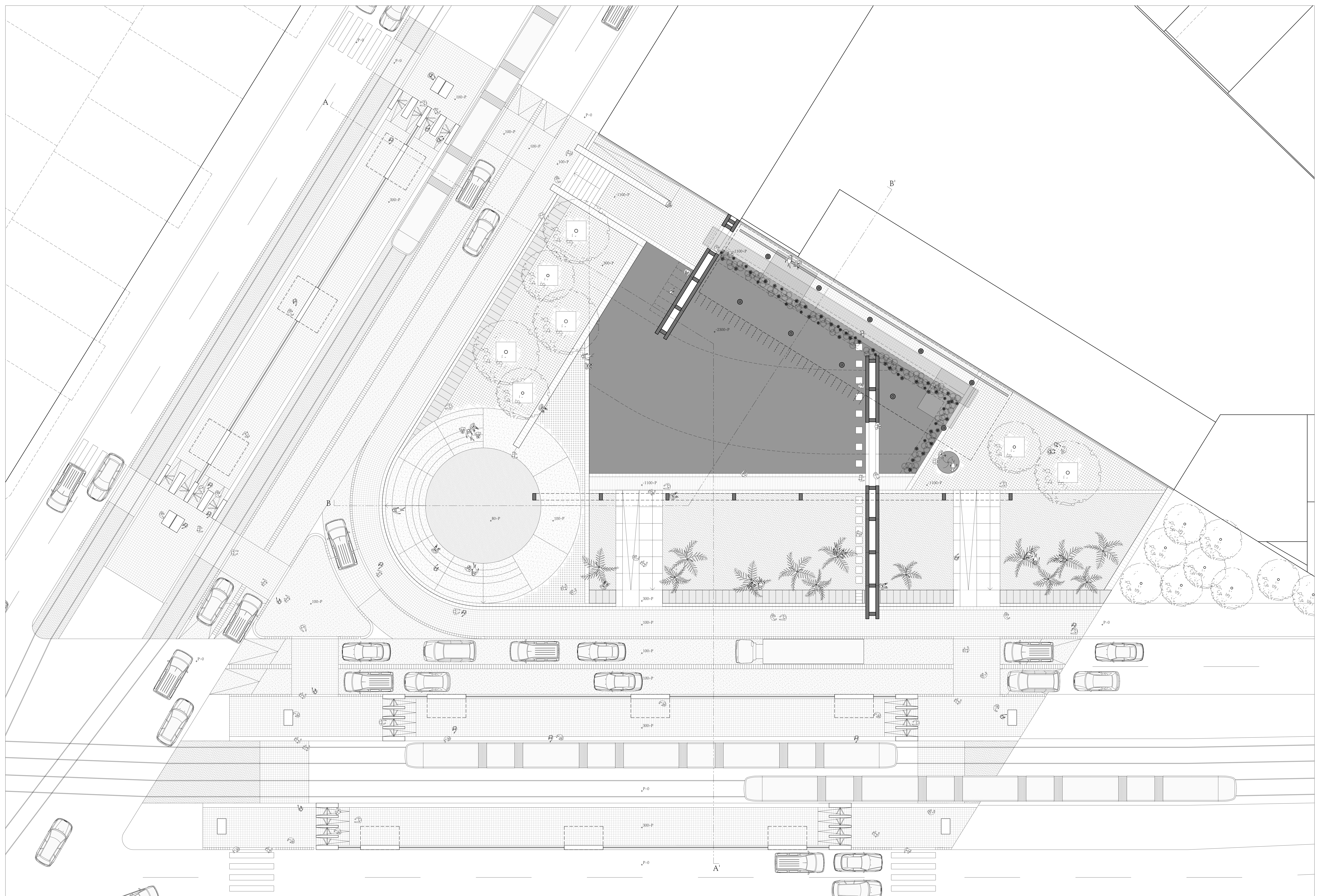
plan . ibn tachfine 1:100
