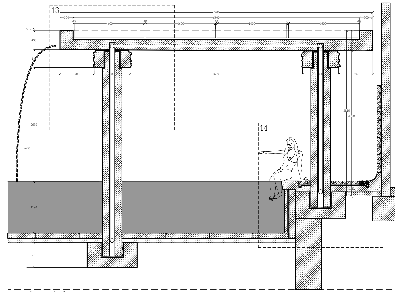
section AA
