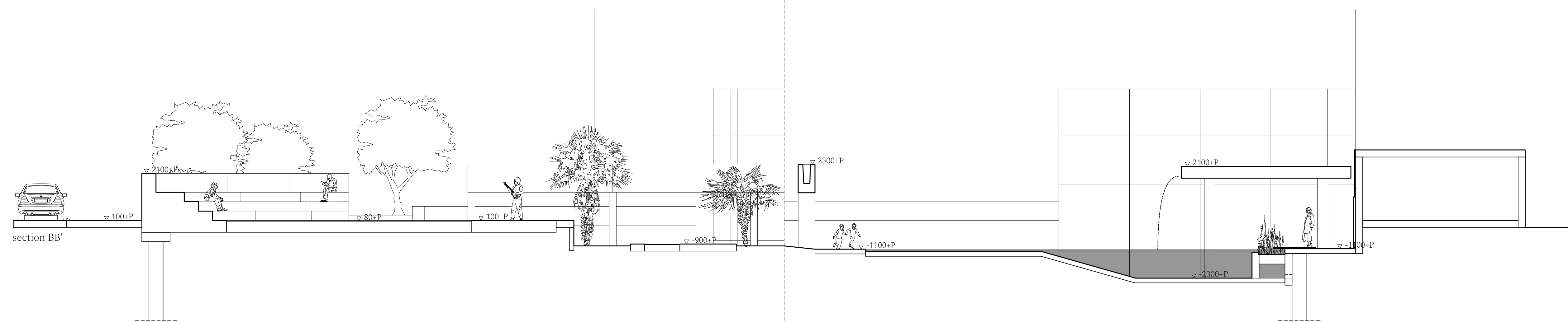
sections . ibn tachfine 1:100
