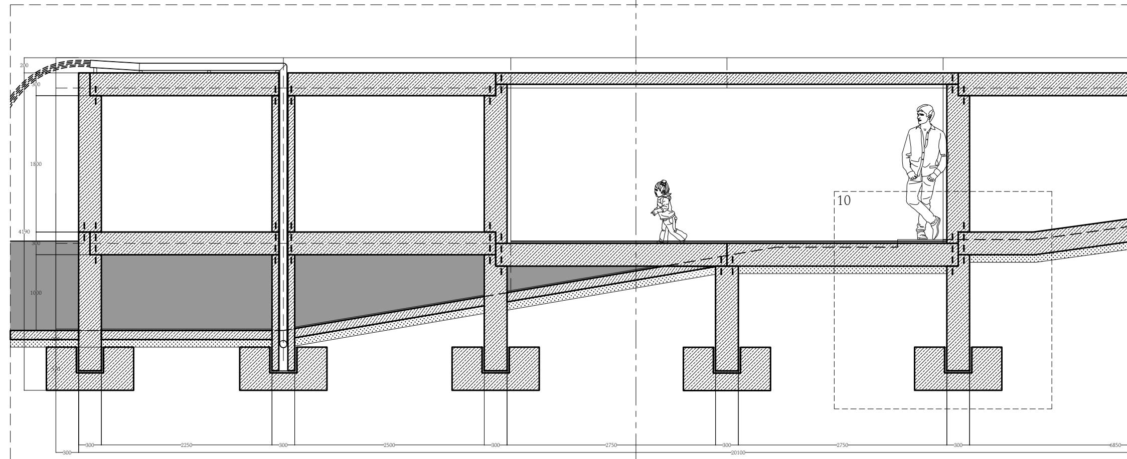
section AA'
