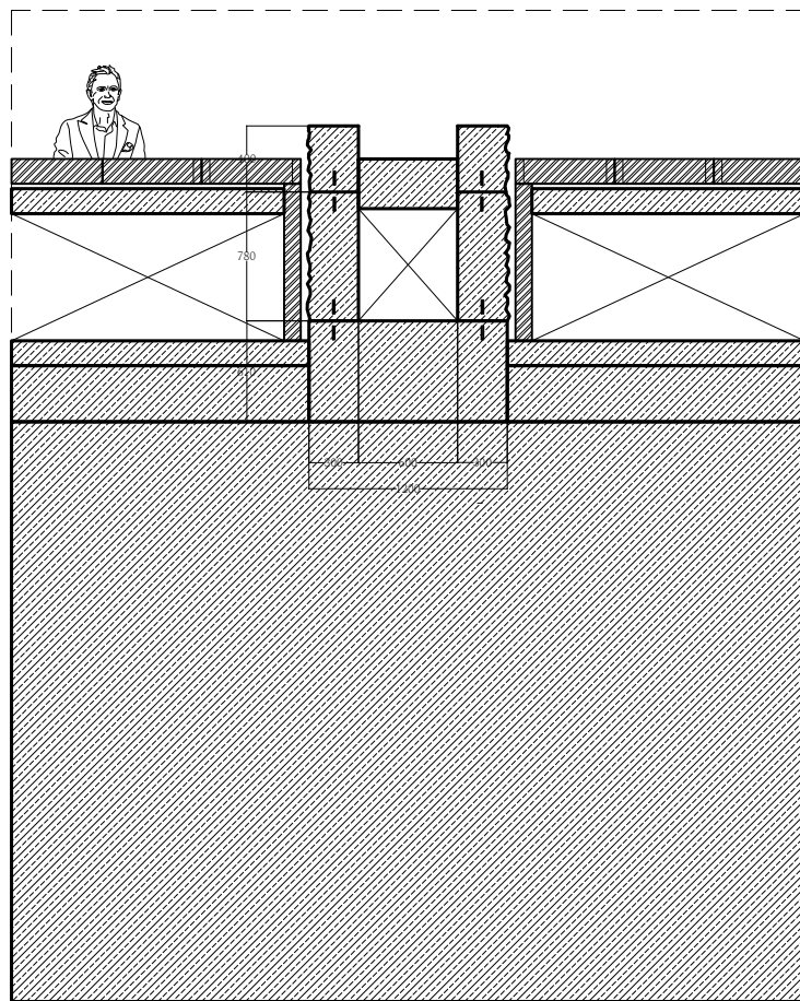
section BB'
