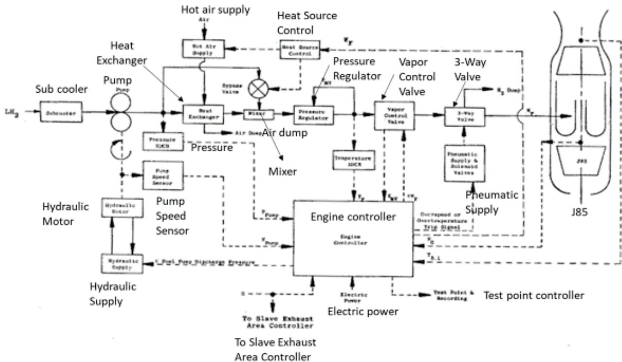
Figure 1. Schematic Diagram of Hydrogen Fuel System. Schematic Diagram of Hyrdogen Fuel System
