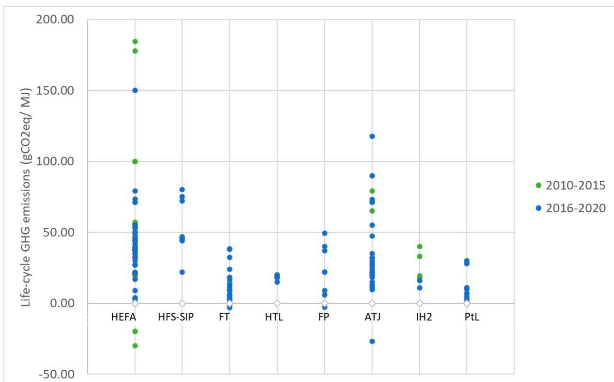
Figure 3-4 Life-cycle GHG emissions for biobased and e-fuel production routes found in the literature with the conventional fuel life-cycle emission as reference. Based on the source: (Capaz et al., 2020; da Silva, 2016; De Jong et al., 2017; O'Connell et al., 2019; Pavlenko et al., 2019; Zemanek et al., 2020), (Patrick Schmidt V. B., 2018), (Lehmann, 2018), (Karl Hauptmeier, Electrofuel / e-Fuel, Production Pathways and Costs , 2018), (Soler, 2019).
