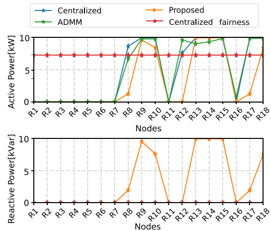
Fig. 8. Required power to regulate the voltage.
