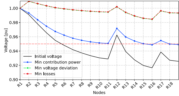
Fig. 7. Voltage profiles before and after voltage regulation with different objectives.
