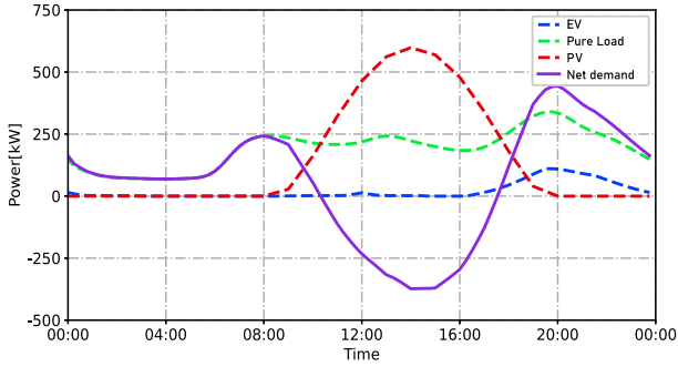
Fig. 6. Active power demand in a typical day.
