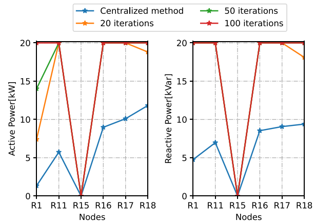
Fig. 16. Required power to regulate voltage with a single agent failure.
