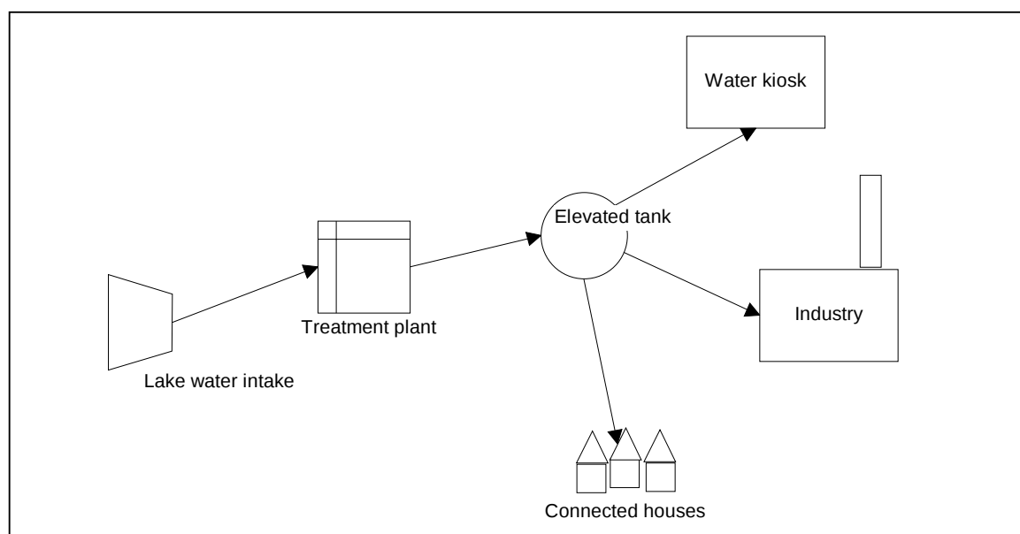
Figure 4.1. Overview existing water supply system in Kisumu
