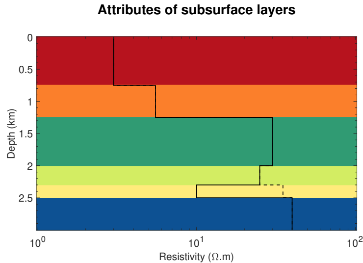
Figure 2 Electric resistivity model as a function of depth where the colours indicate the resistivity that is shown in the black line; the values that belong to the colours can be read off from the horizontal axis. The dashed line marks the time-lapse change.
