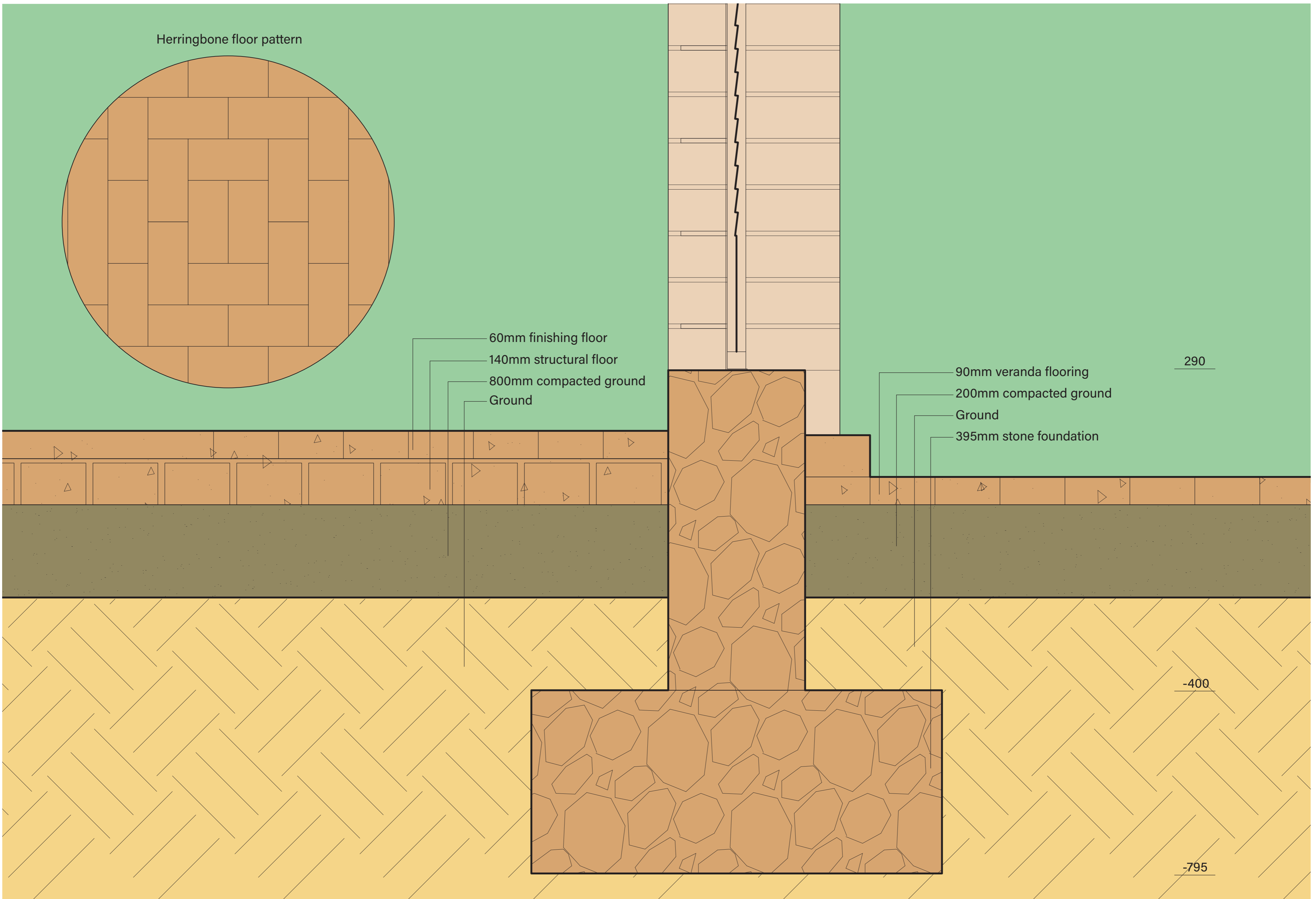
FOUNDATION DETAIL | 1:5
