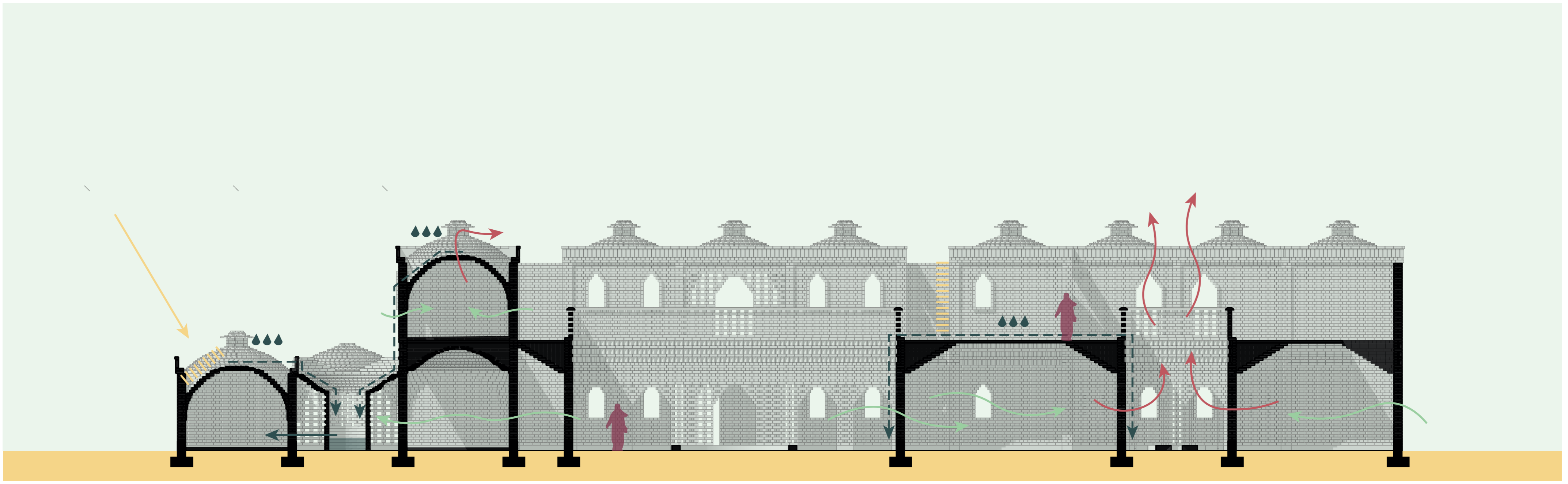
CLIMATE SECTION | 1:100
