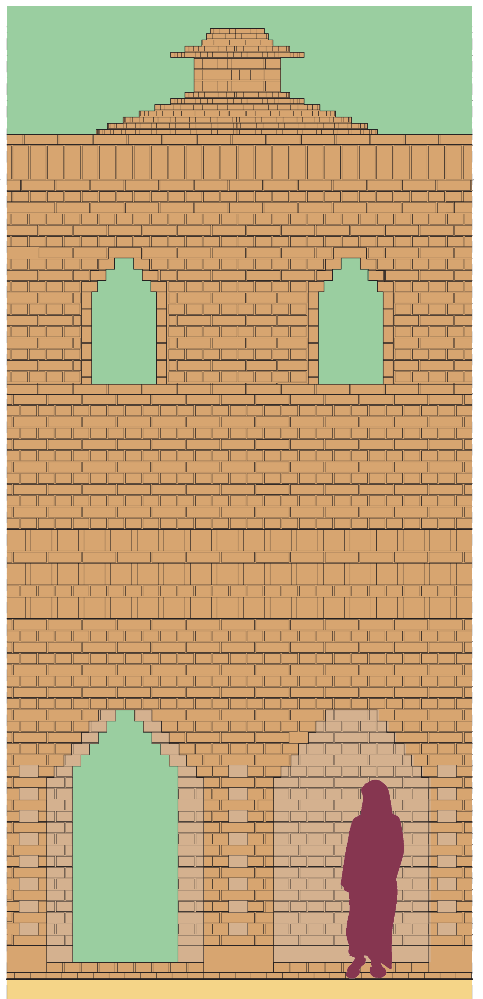
FACADE FRAGMENT | 1:20
