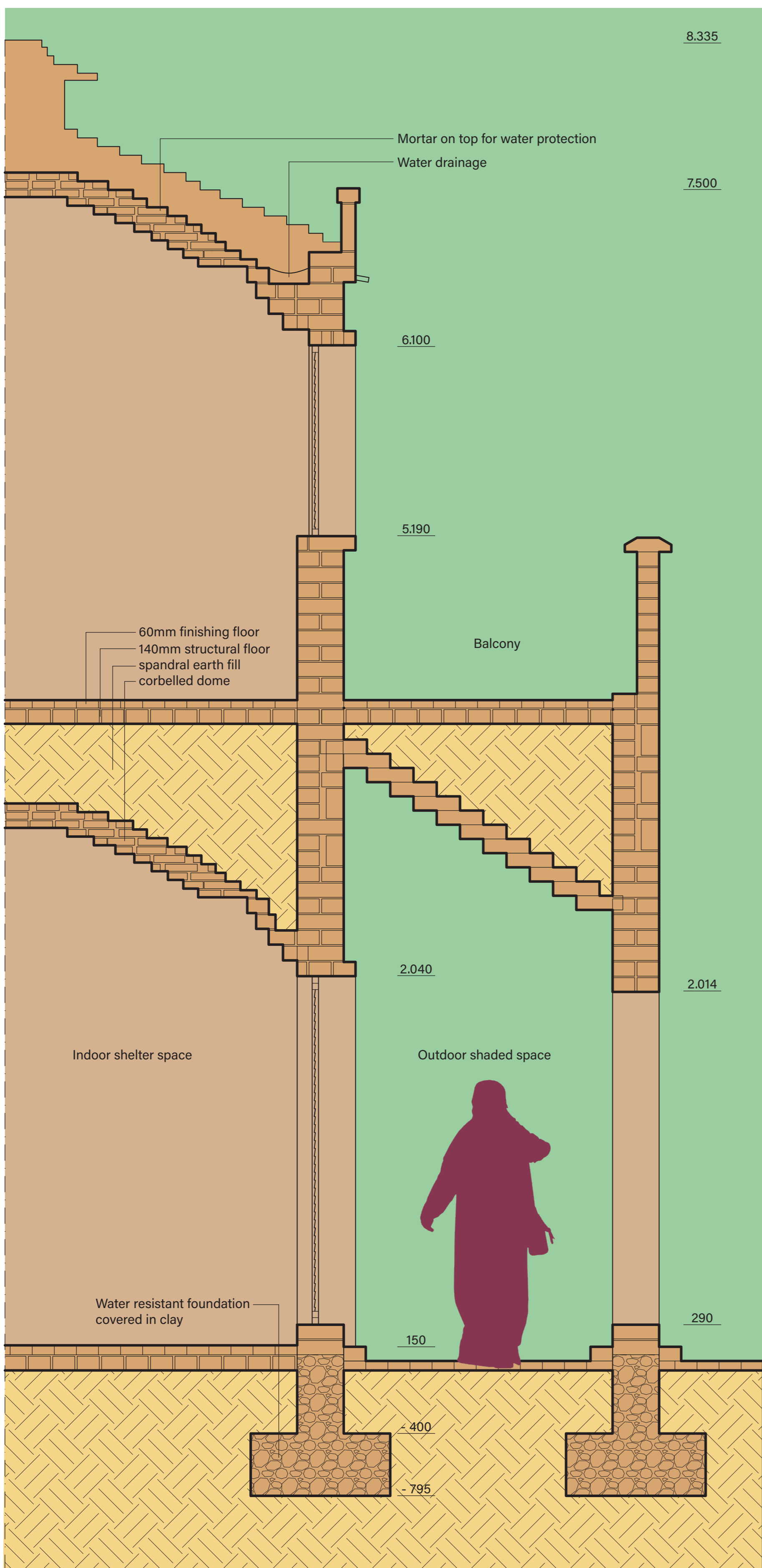
SECTION FRAGMENT | 1:20
