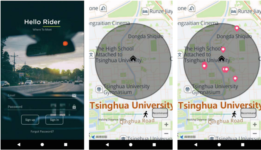
(a) Login (b) Input pick-up location and walking distance (c) Recommend a set of pick-up locations
