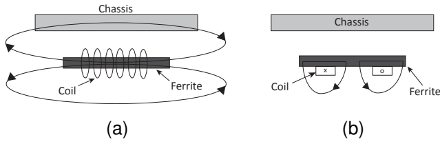
Figure 1. Classification of coupler topologies based on the strategy of coil winding: (a) double-sided winding, (b) single-sided winding.
