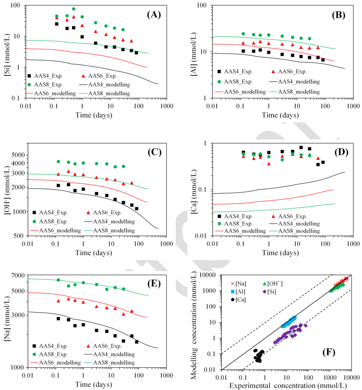
Fig. 14. Modelled elemental concentrations in comparison with the experimental measurements. (A) [Si]; (B) [Al]; (C) [OH - ]; (D) [Ca], (E) [Na] and (F) modelling concentration versus experimental concentration regardless of time and Na 2 O content. In the graphs, AAS indicates alkali-activated slag, and the number following AAS refers to the weight percentage of Na 2 O with respect to slag. Exp. is abbreviated from experimental. Water to slag ratio was 0.4 and the curing temperature was 20 °C.
