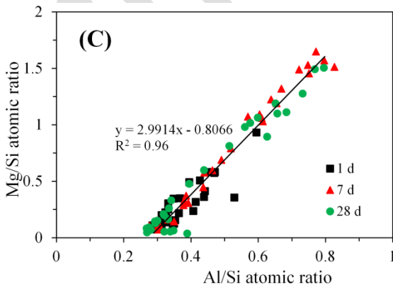
Fig. 8. Atomic ratios Mg/Si versus Al/Si for AAS4 (A), AAS6 (B) and AAS8 (C) at 1, 7 and 28 days. AAS indicates alkali-activated slag, and the number following AAS refers to the weight percentage of Na 2 O with respect to slag. Water to slag ratio was 0.4 and the curing temperature was 20 °C.
