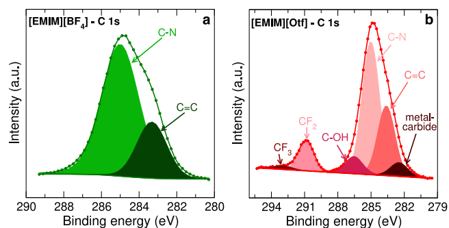
Fig. 4. Normalized C 1s XPS spectra of VS-MoS 2 catalyst exposed to [EMIM][BF 4 ] (a) and to [EMIM][Otf] (b).
