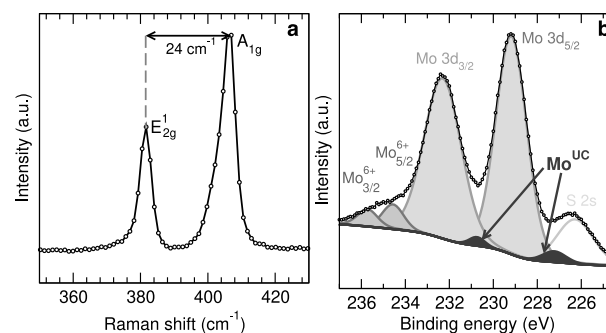
Fig. 1. (a) Raman spectrum of the V S -MoS 2 catalyst showing the two characteristic peaks, E 2g 1 and A 1g of the material, (b) Fitted Mo 3d5 XPS spectrum of the V S -MoS 2 catalyst showing the different valence states of the Mo atoms in the structure.
