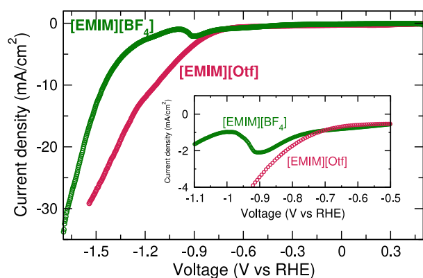
Fig. 2. Linear sweep voltammetry curves of the MoS 2 catalyst in [EMIM][BF 4 ]-water mixture (green) and [EMIM][Otf]-water (red) mixture.
