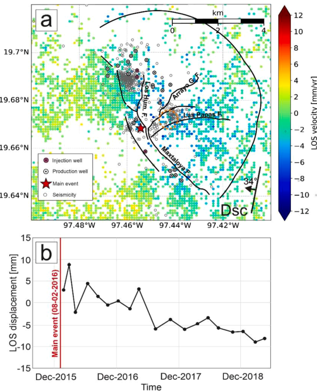
Figure 5. (a) Mean PS velocities in mm/year in the direction of the satellite line of sight (LOS) at the LHGF, observed on descending satellite orbits, after the Mw 4.2 event. Only PS points with a standard deviation <2 mm/year are included. Negative LOS velocities indicate movement away from the satellite ( \sim subsidence) and positive values indicate movement towards the satellite ( \sim uplift). The main structures modified after Calcagno et al. (2018), Norini et al. (2019), the wells operating during the period of the InSAR time series (19 February 2016 – 16 May 2019) and the natural and induced earthquakes between 2017 September and 2018 September after Gaucher et al. (2019) are also shown. (b) Time series plot of the mean LOS velocities from vicinity of the Las Papas fault, highlighted in (a) with the dashed orange circle.
