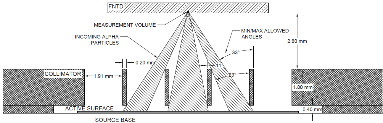
Figure 3: Schematic overview of possible alpha tracks through a 1.8 mm (1800 \mu\text{m} ) thick collimator entering the measured area of the FNTD at position 1 (see Fig. 4). A total of 9 irradiations positions were chosen to represent the angular distribution of the whole irradiation field. Note that since a total of 9 positions are used for the irradiation of FNTDs, the collective angular distribution of alpha tracks measured in the FNTDs will yield an angular distribution with less pronounced peaks than found when
