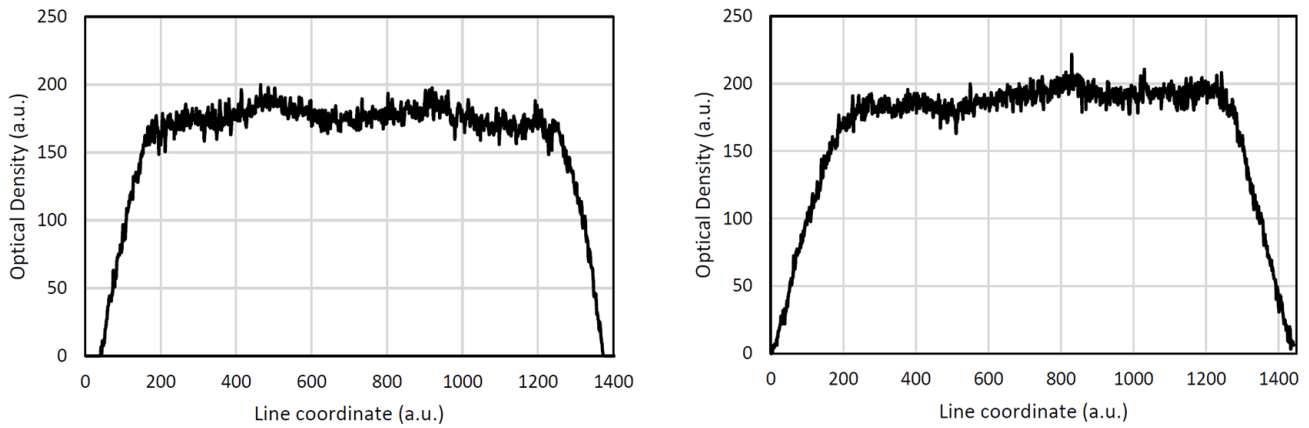
Figure 7: Contrast enhanced optical density maps of Gafchromic tm HD-V2 film irradiated using the 1800 \mu\text{m} (left) and 2600 \mu\text{m} (right) collimator.
