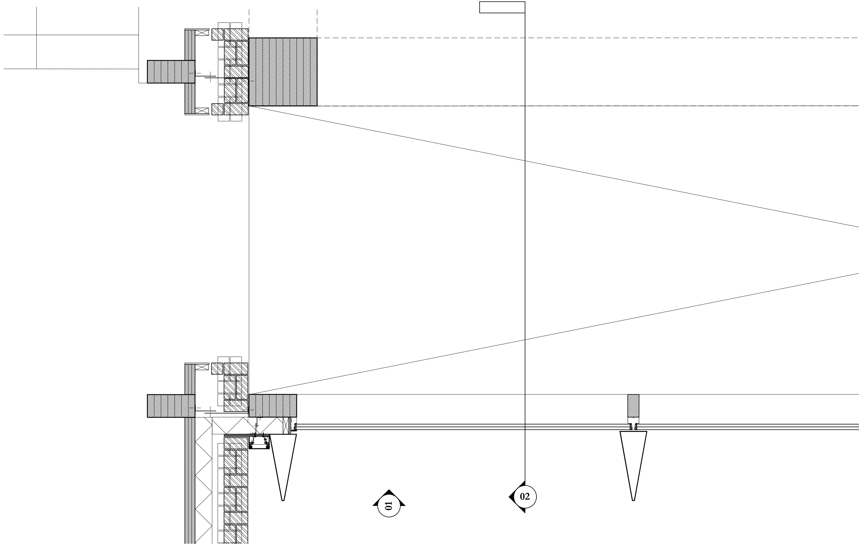
04 Public Hall Lower Detail Plan
