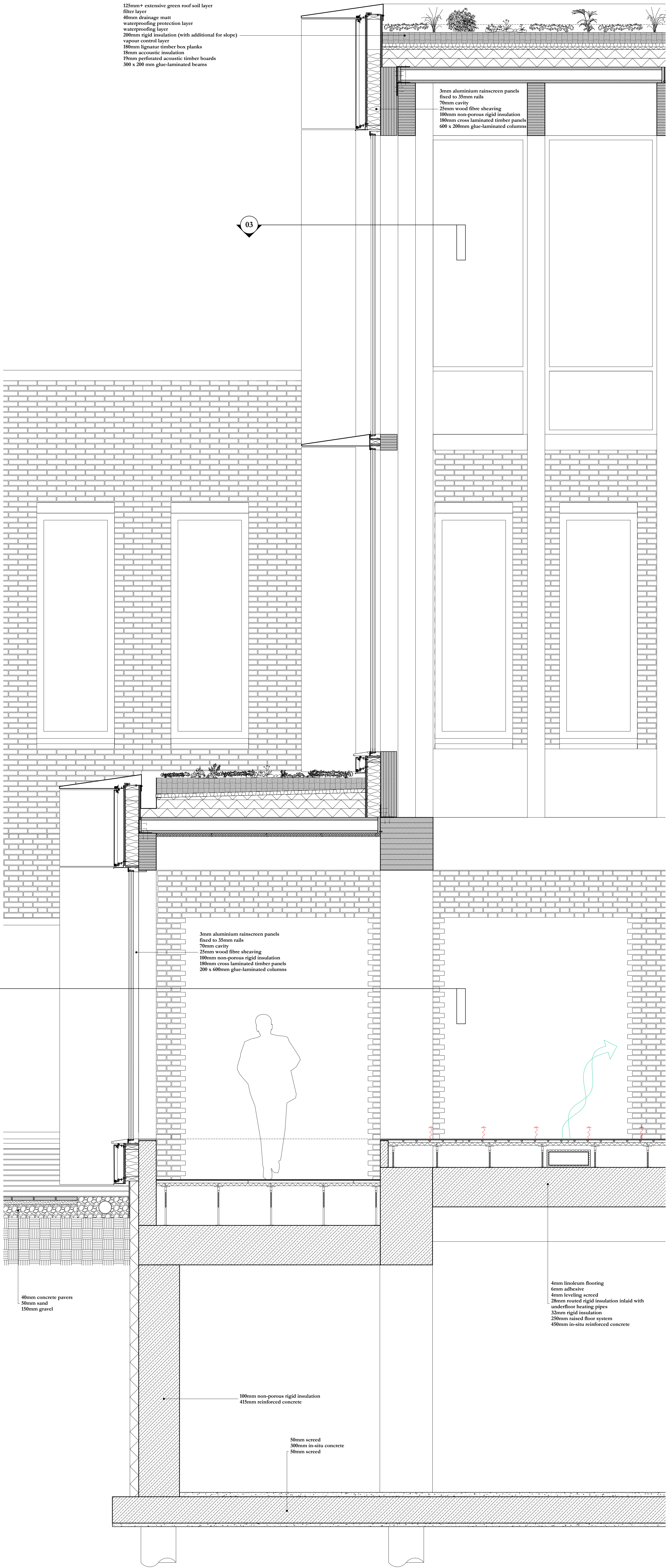
02 Public Hall Detail Section
