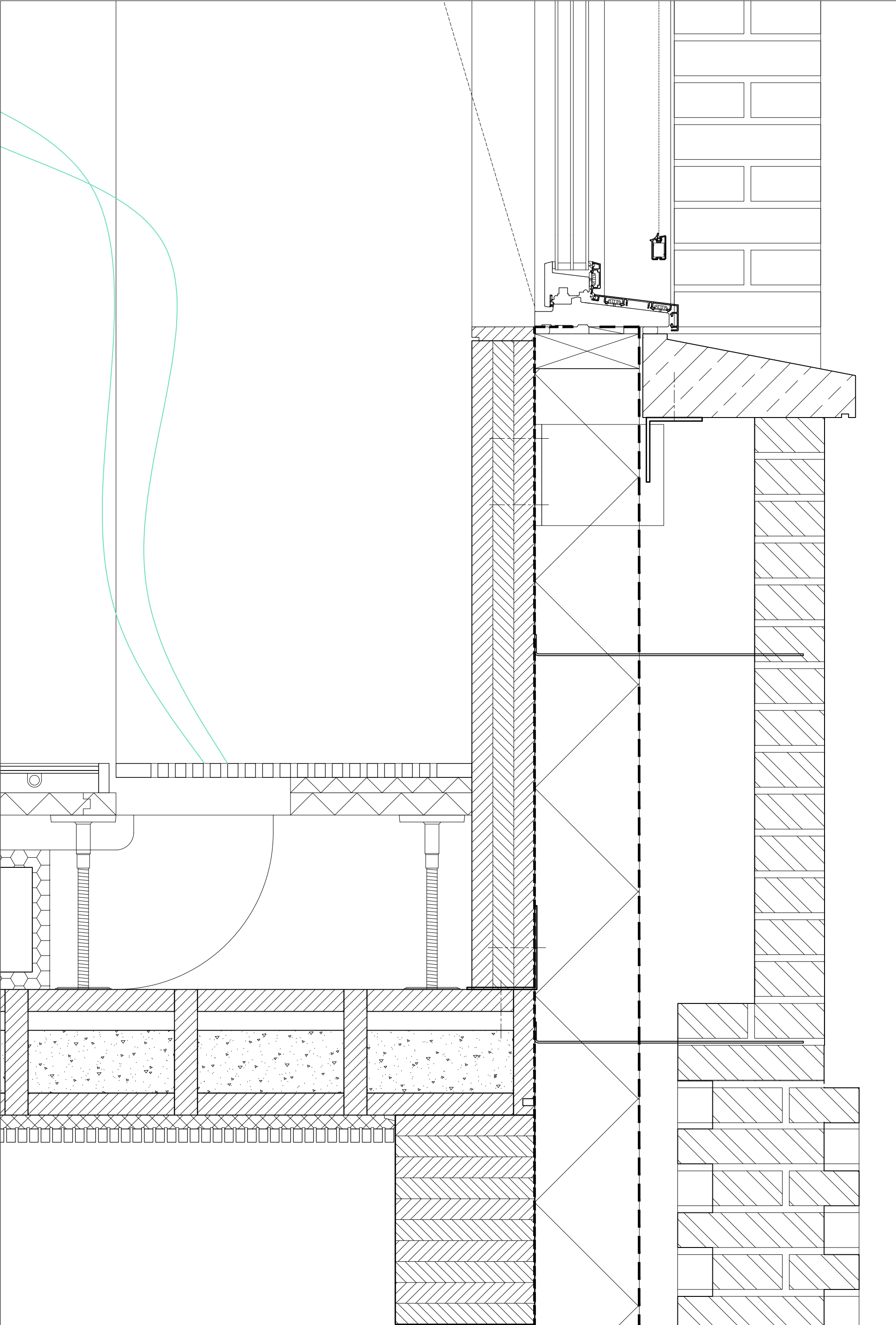
D2 Front Facade Window Cill Detail 0 0.5m
