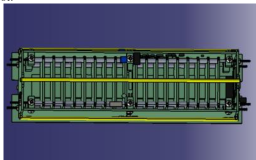
Figure 4 1-stack
