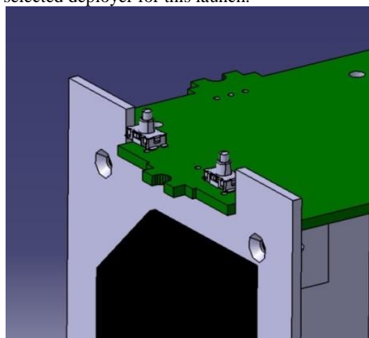
Figure 6 Deployment switches
