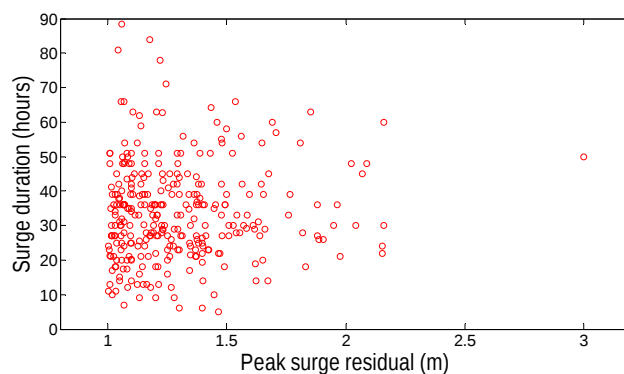
Fig. 5. The peak surge residuals and associated durations.
