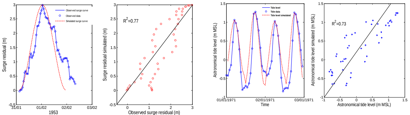
Fig. 8. The stochastic astronomical tide function.
