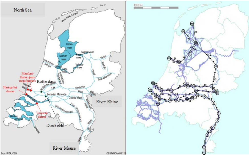
Fig. 2. (left) Description of the Rhine delta with existing operated structures and (right) overview of the simplified 1-D hydrodynamic model (van Overloop, 2009).
