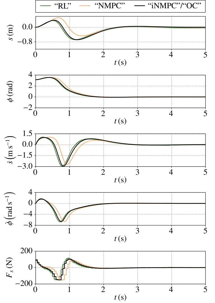
Figure 3: State and control trajectories obtained by the frozen methods for the cart-pendulum system without uncertainties. For “RL” the mean and standard deviation of 50 trajectories is shown. Y-axes variables s, \dot{s} denote the cart position and velocity and \phi, \dot{\phi} are the respective quantities of the pendulum. F_s is the force acting on the cart body.
