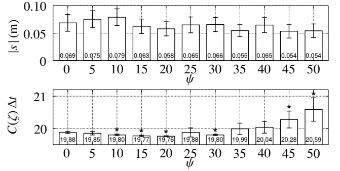
Figure 5: Influence of the shaping function on the results of the “RL” method. Top: absolute error in the cart position at the end of an episode depending on the weight \psi of the shaping function. Bottom: total cost of the trajectory. Shaping is not used for \psi = 0 . Numbers inside of the bars show the mean value of the error averaged over 50 independent runs, while the error bars show the upper and lower 95% confidence limits. Statistically significant result, for which the p-value is less than 0.05, is marked with * above the bars.
