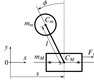
Figure 2: The inverted pendulum on a movable cart.
